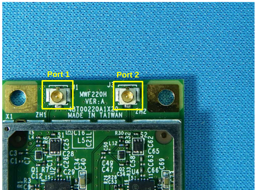
Antenna Port
