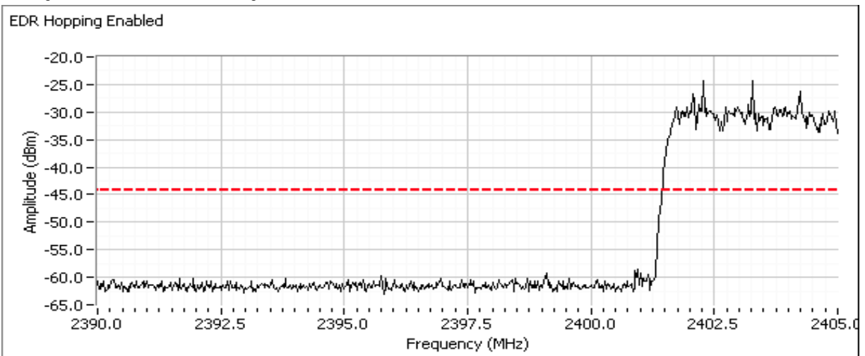
Plot showing -20dBc at the lower band edge
