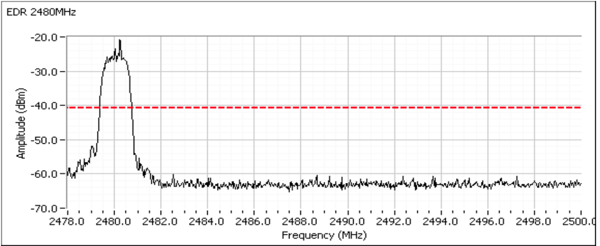
Plot showing -20dBc at the upper band edge
