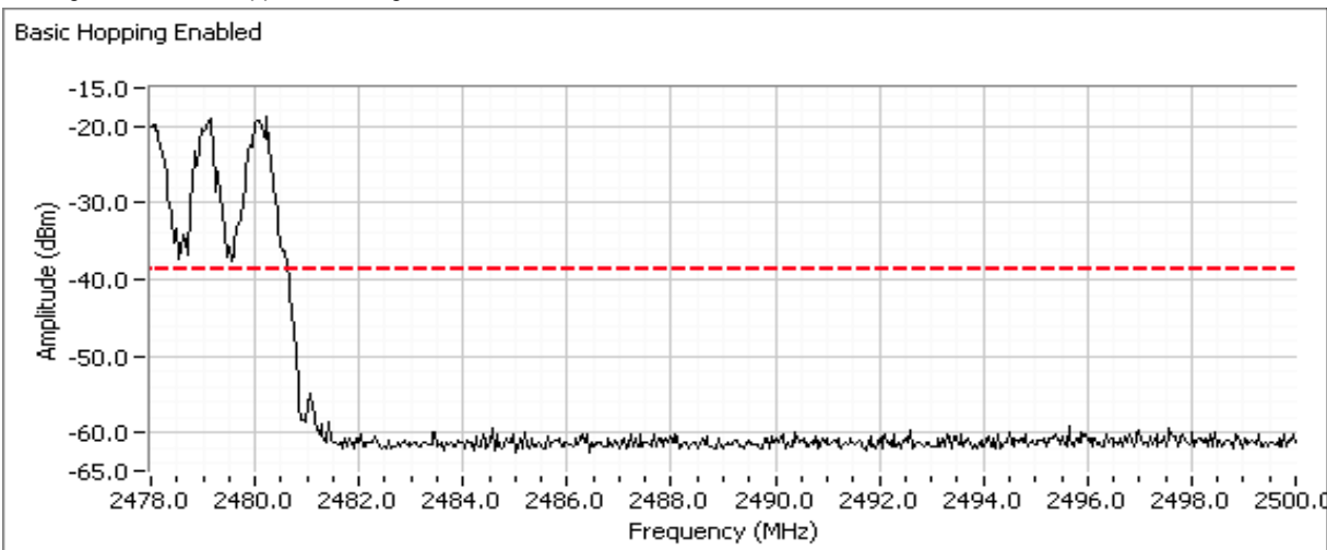
High channel, hopping enabled Plot showing -20dBc at the upper band edge
