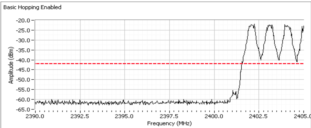
Low channel, hopping enabled Plot showing -20dBc at the lower band edge
