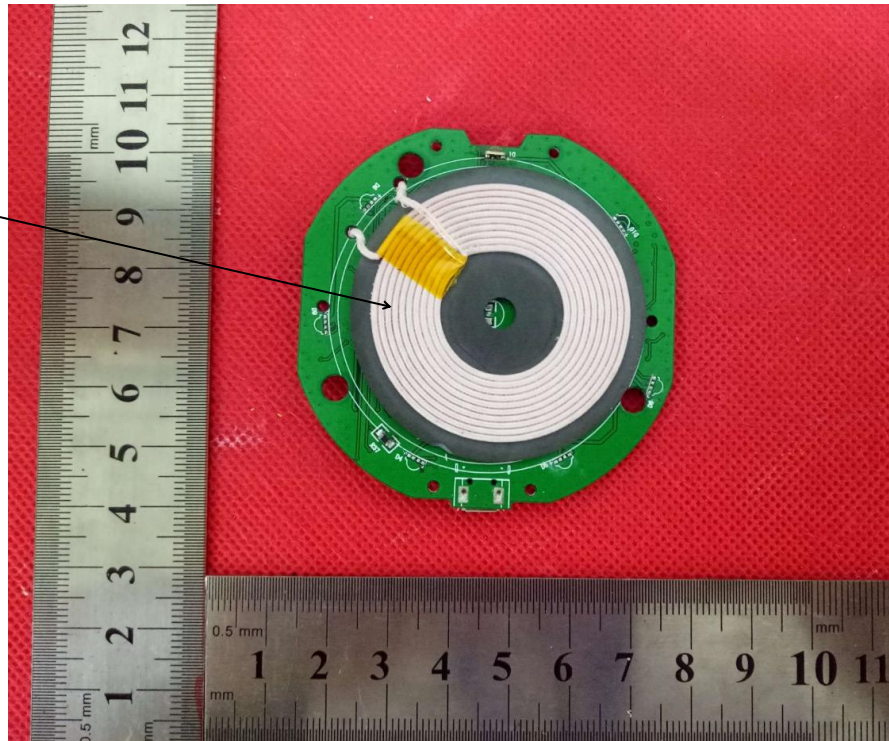
Coil Antenna
