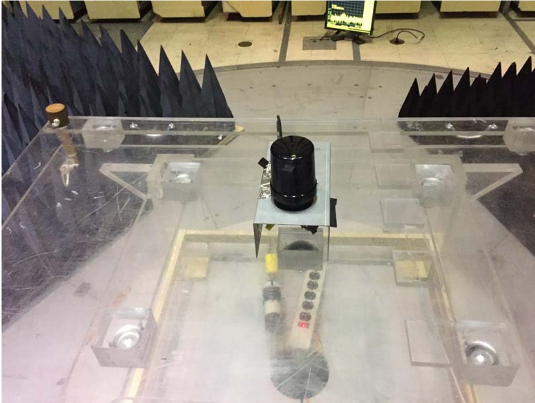
Radiated Spurious and Fundamental Power; front, up to 18 GHz
