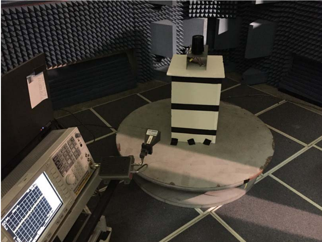
Radiated Spurious 18-25 GHz
