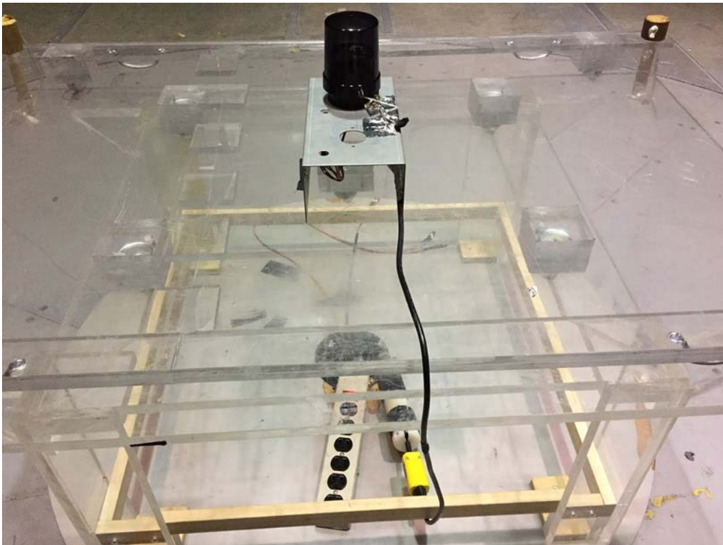
Radiated Spurious and Fundamental Power; back, up to 18 GHz
