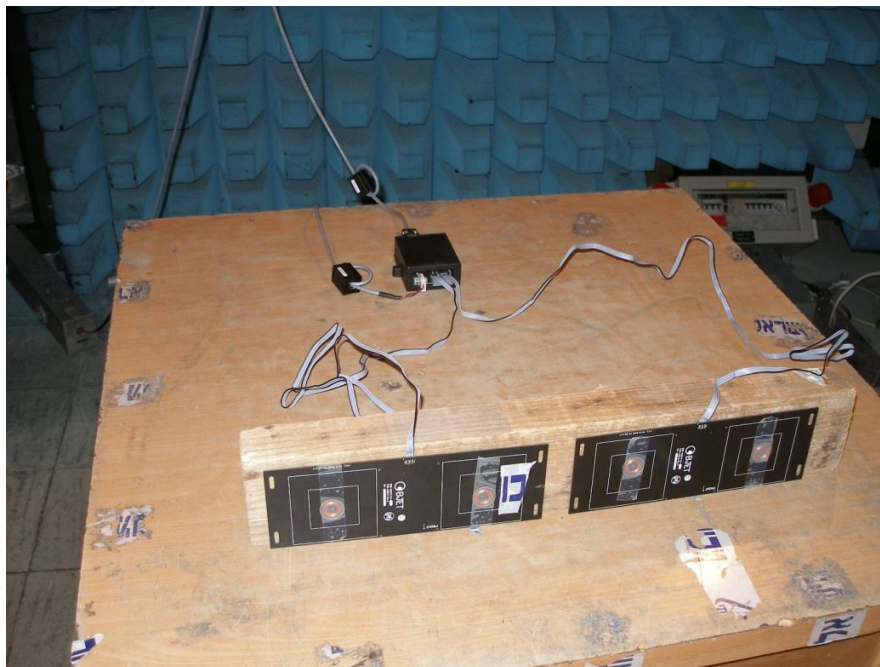
Photo 2. RE test setup in Anechoic chamber.
