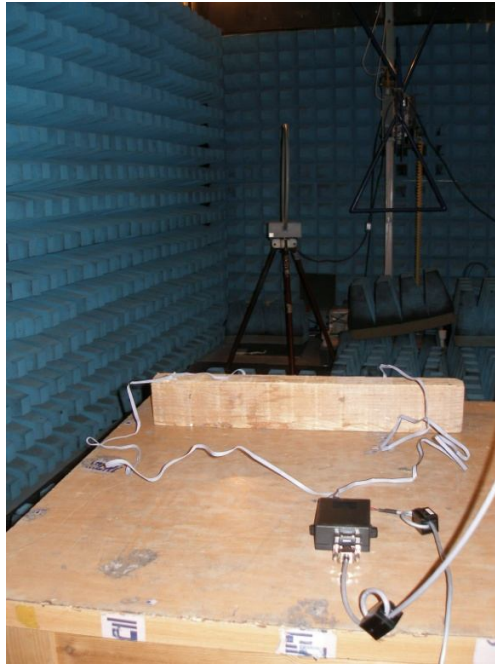
Photo 1. RE test setup in Anechoic chamber with loop antenna.
