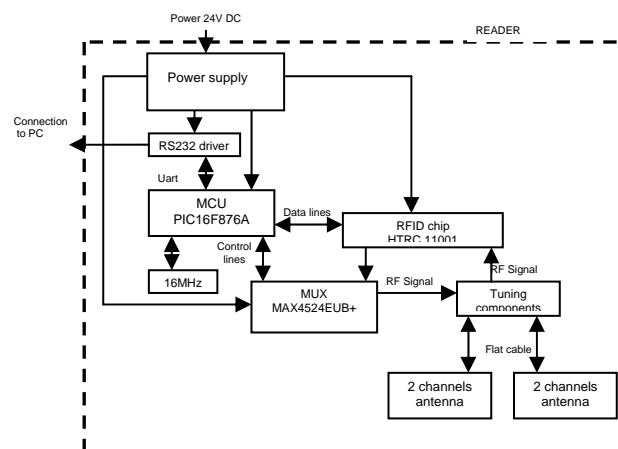
Figure 1. The RFID unit block-diagram.
