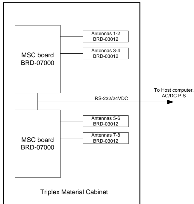
Figure 3. RE test setup block diagram.
