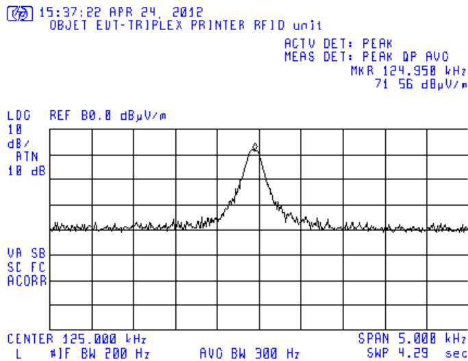
Plot # 1. Field strength of fundamental frequency 125 kHz.
