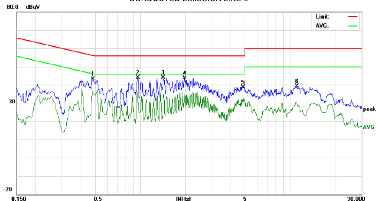
CONDUCTED EMISSION LINE-L
