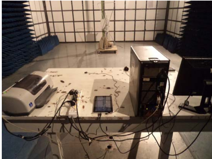
Radiated Emission 30MHz To 1G
