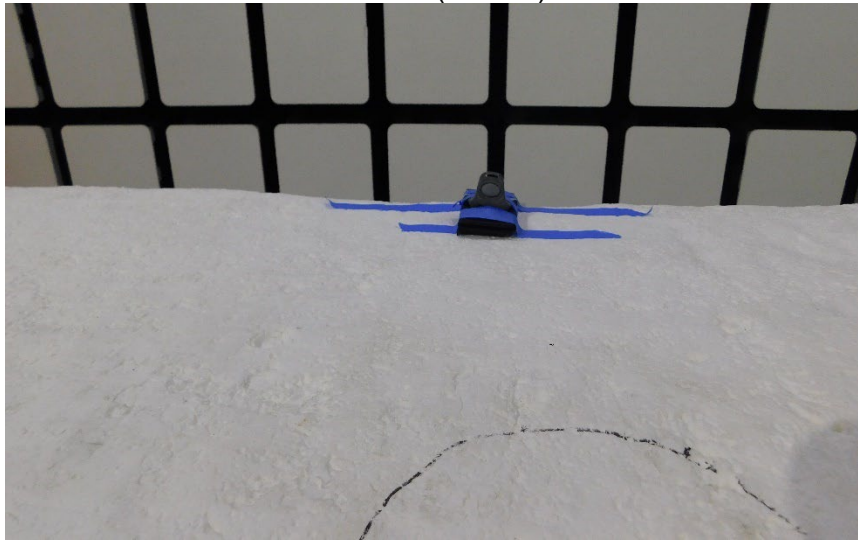
RADIATED SPURIOUS PHOTO (>1GHz)
