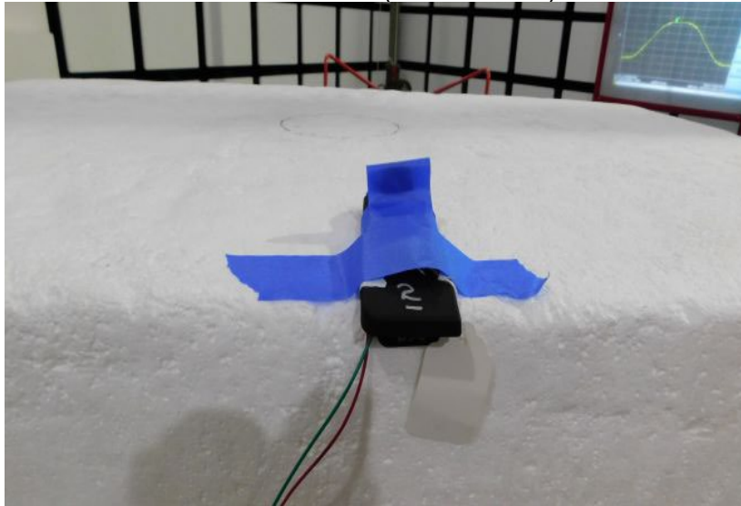
RADIATED SPURIOUS PHOTO (X Orientation)
