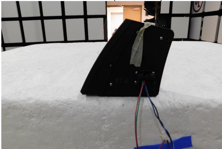
RADIATED SPURIOUS PHOTO (Y Orientation)
