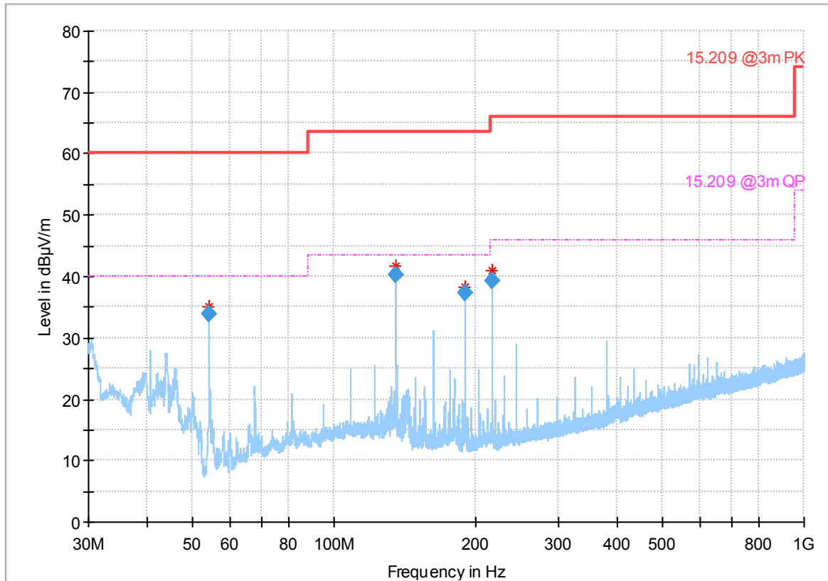
Plot no. 5: Radiated emissions 30 MHz – 1 GHz, hor./vert. polarization, Left handle, lying
