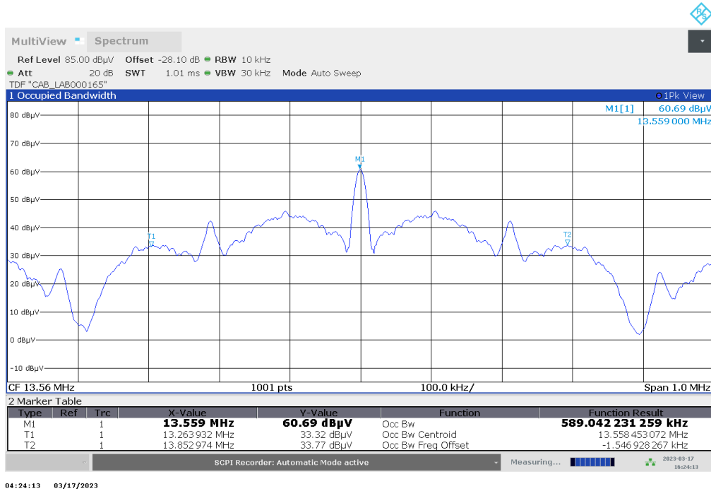
Plot no. 15: Frequency tolerance @ +85 °C, Left handle, Vmax
