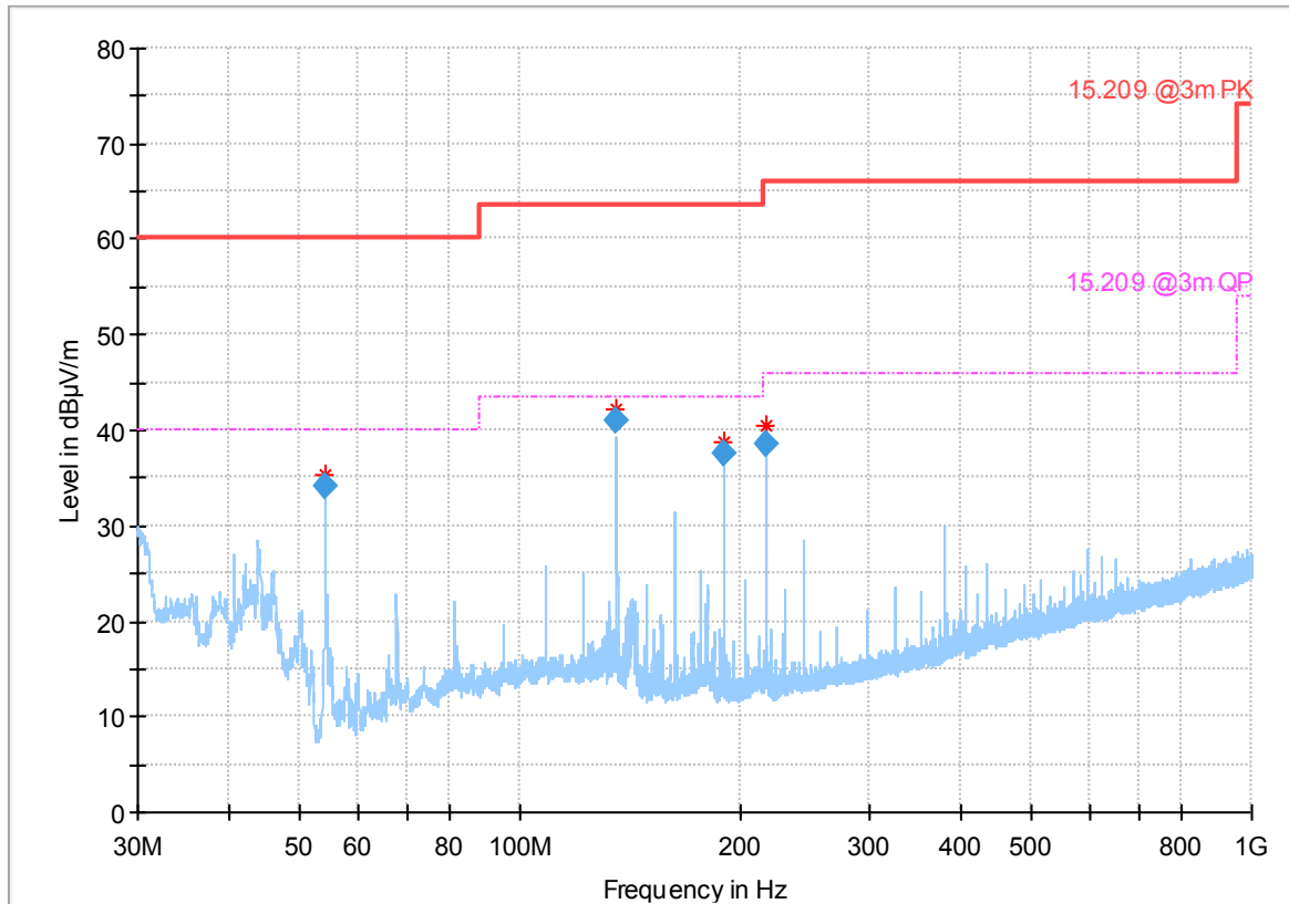
Plot no. 6: Radiated emissions 30 MHz – 1 GHz, hor./vert. polarization, Left handle, staying
