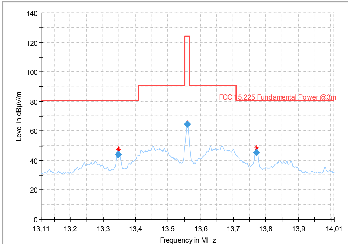
Plot no. 1: Transmitter Spectrum Mask (TSM), Left handle, lying
