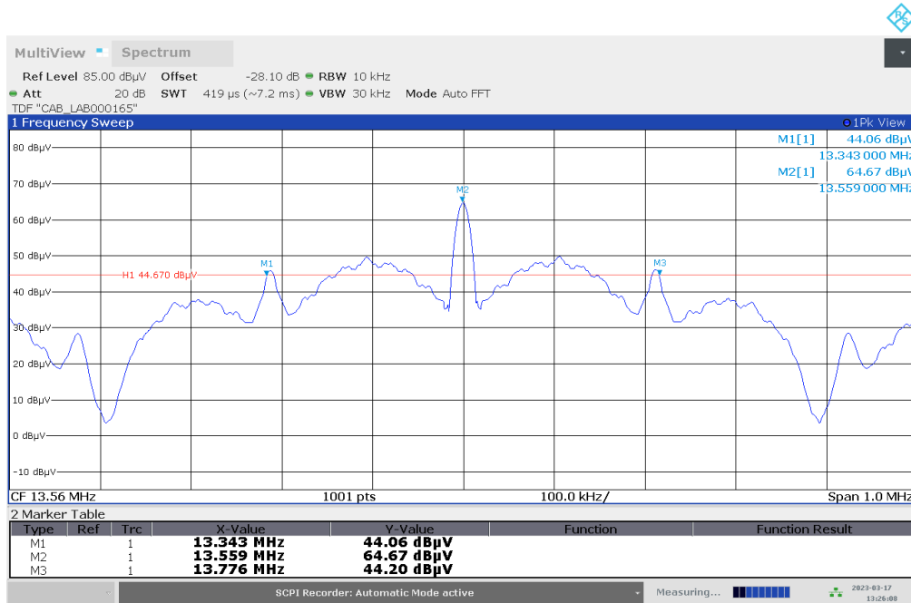
Plot No. 17: 20 dB bandwidth, Left handle
