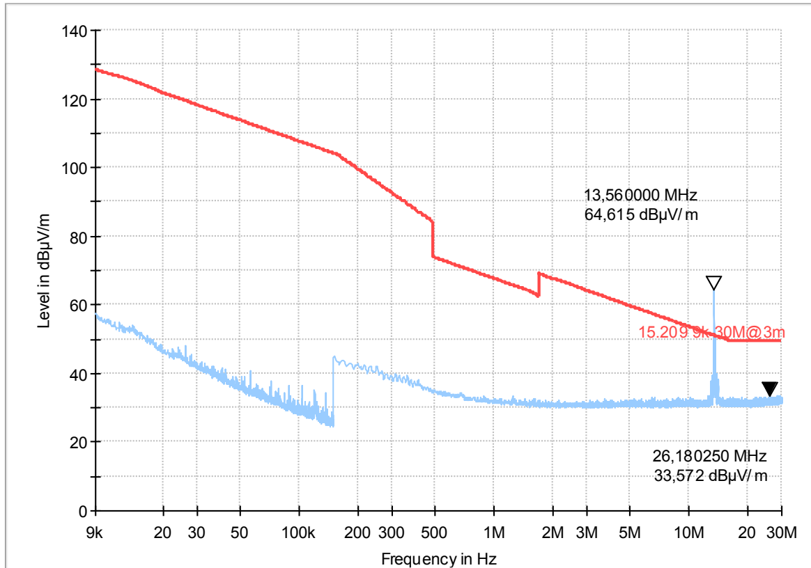
Plot no. 3: Radiated emissions 9 kHz – 30 MHz, Left handle, lying
