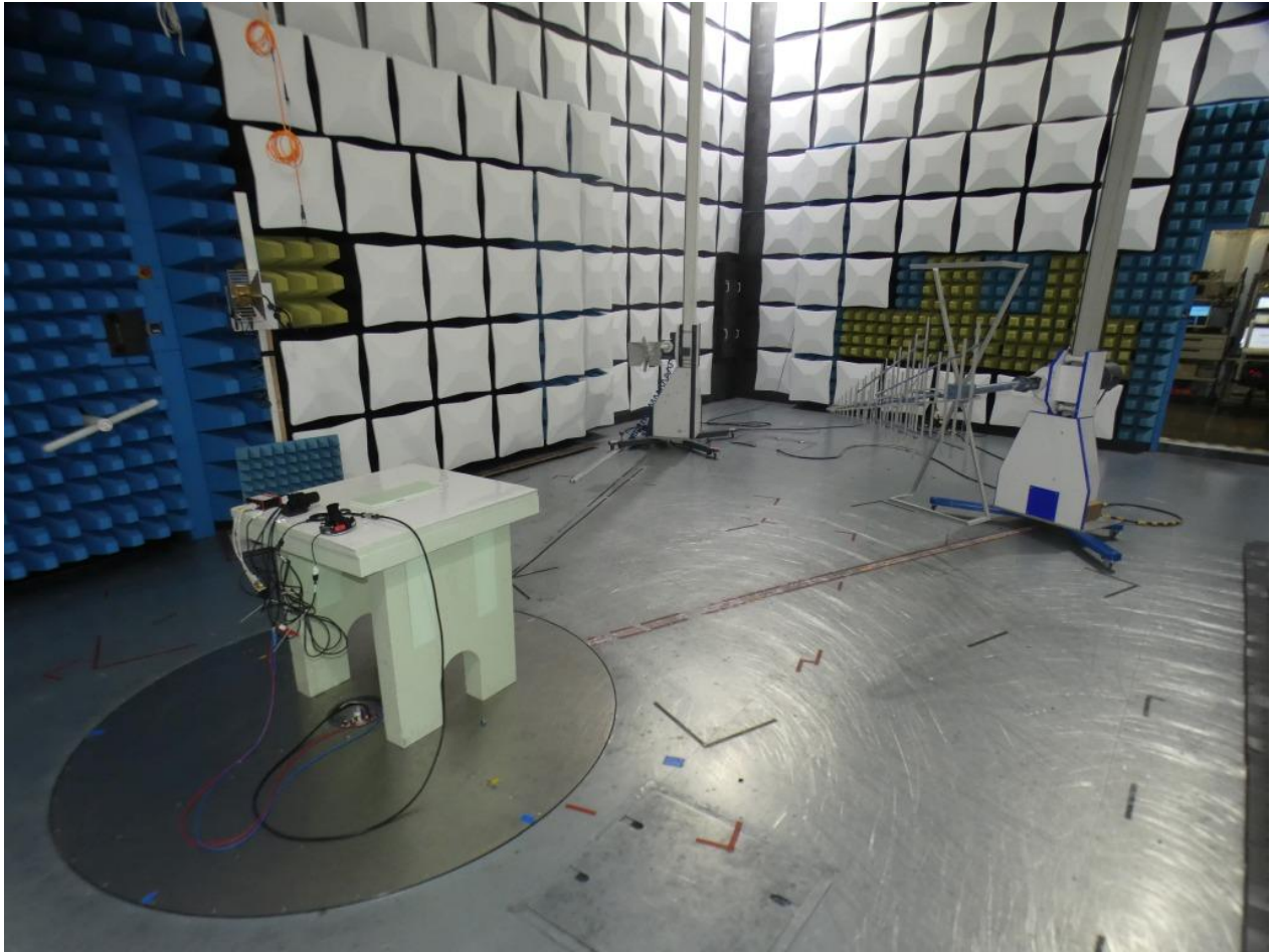
Photo 2: Test setup for radiated measurements (30 MHz - 1 GHz)
