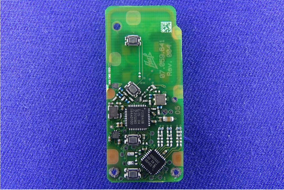
(22) EUT Photo
