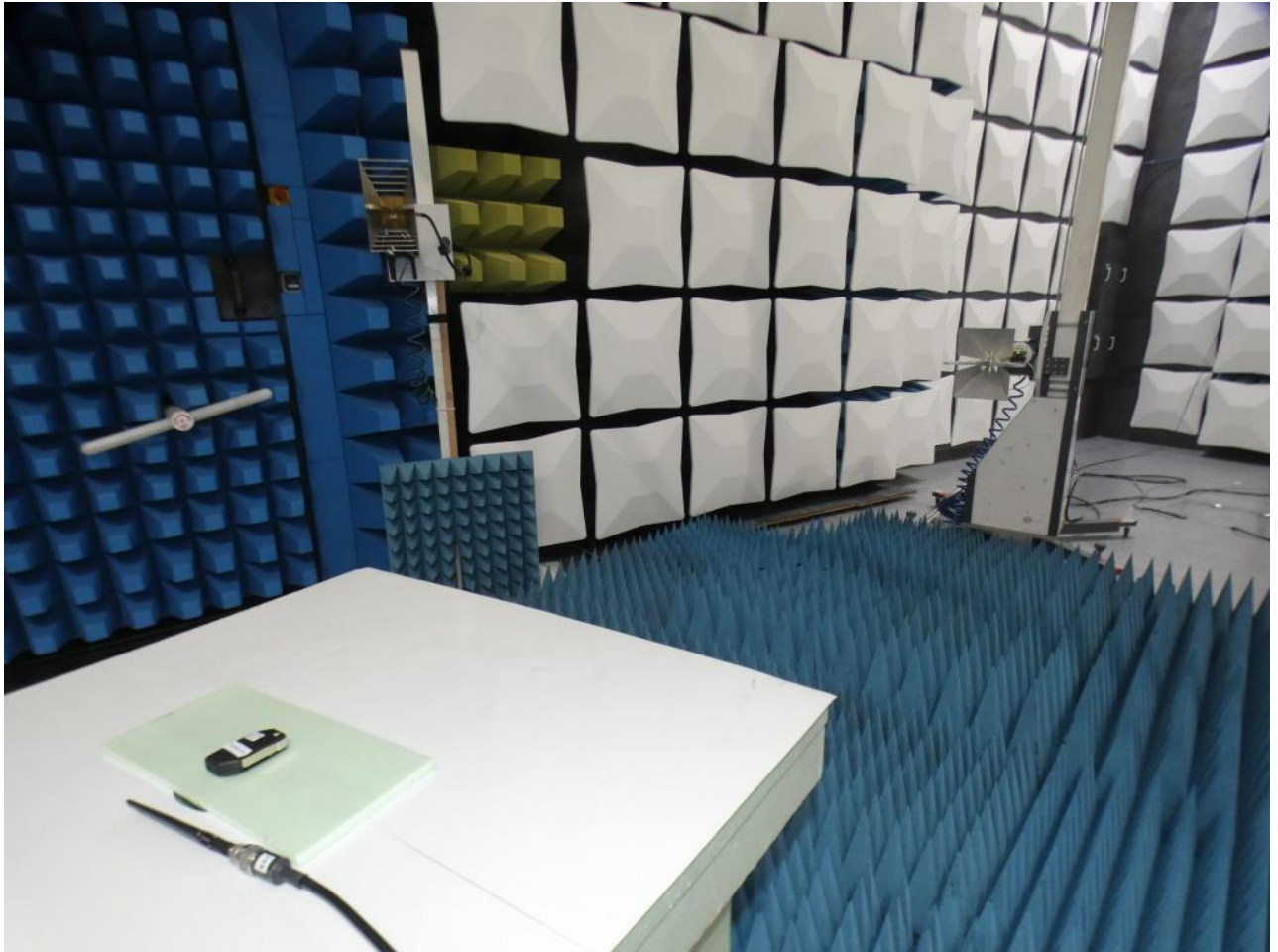
Photo 3: Test setup for radiated measurements (1 GHz – 5 GHz)
