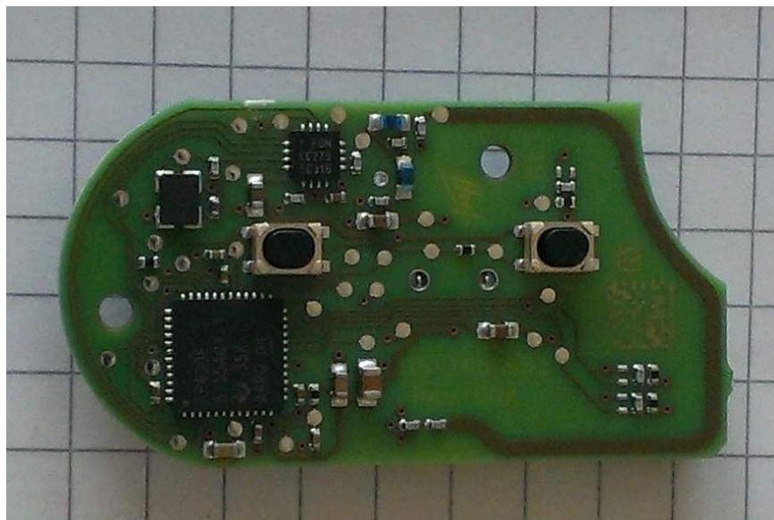
Pic. 4 PCB top view
