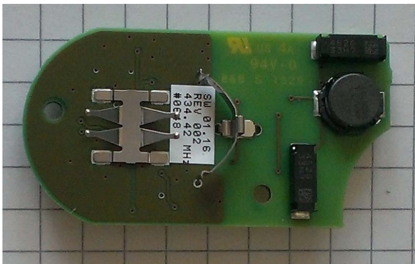
Pic. 5 PCB rear view
