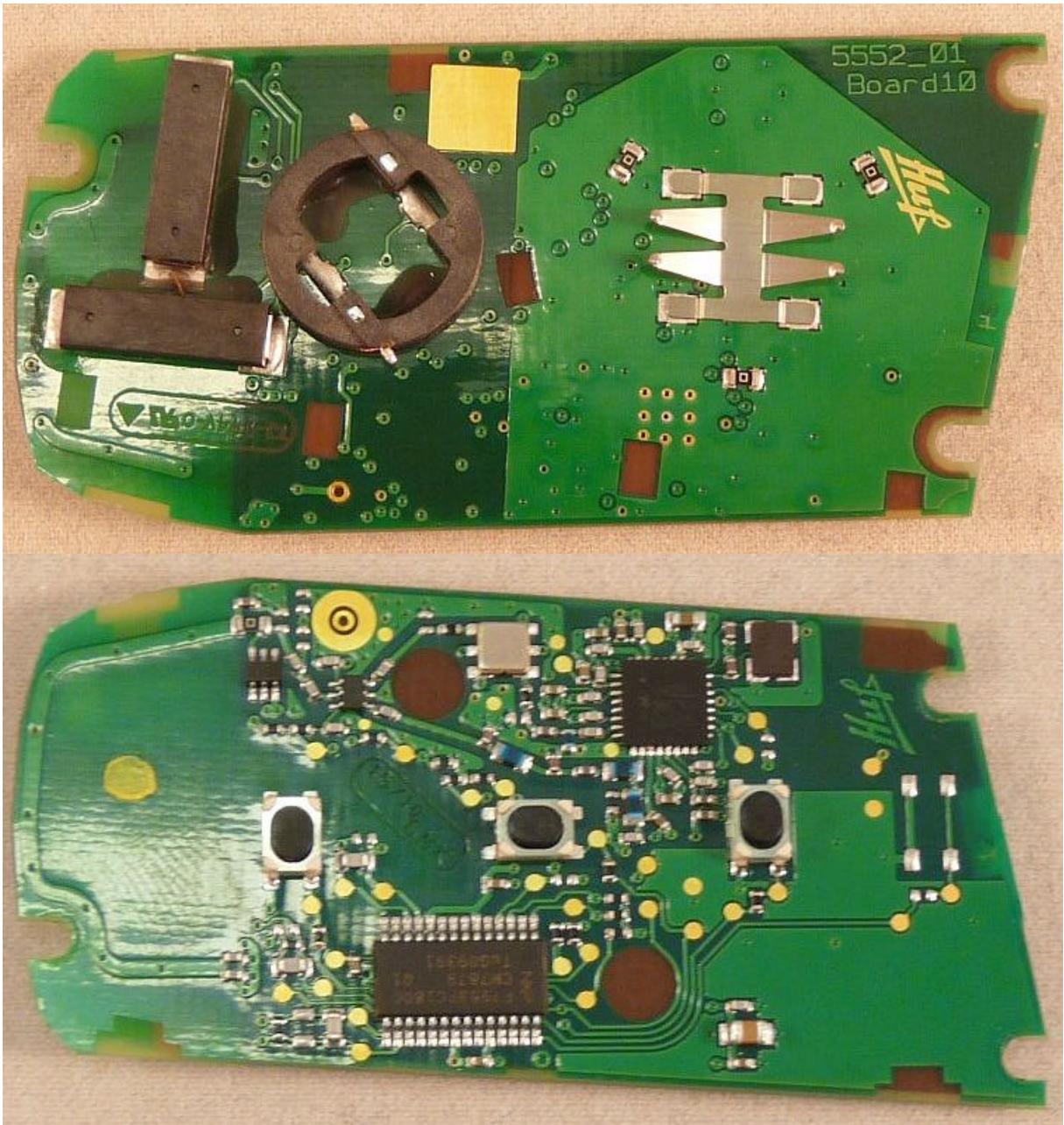
Photo 5: PCB of EUT (front and rear view)
