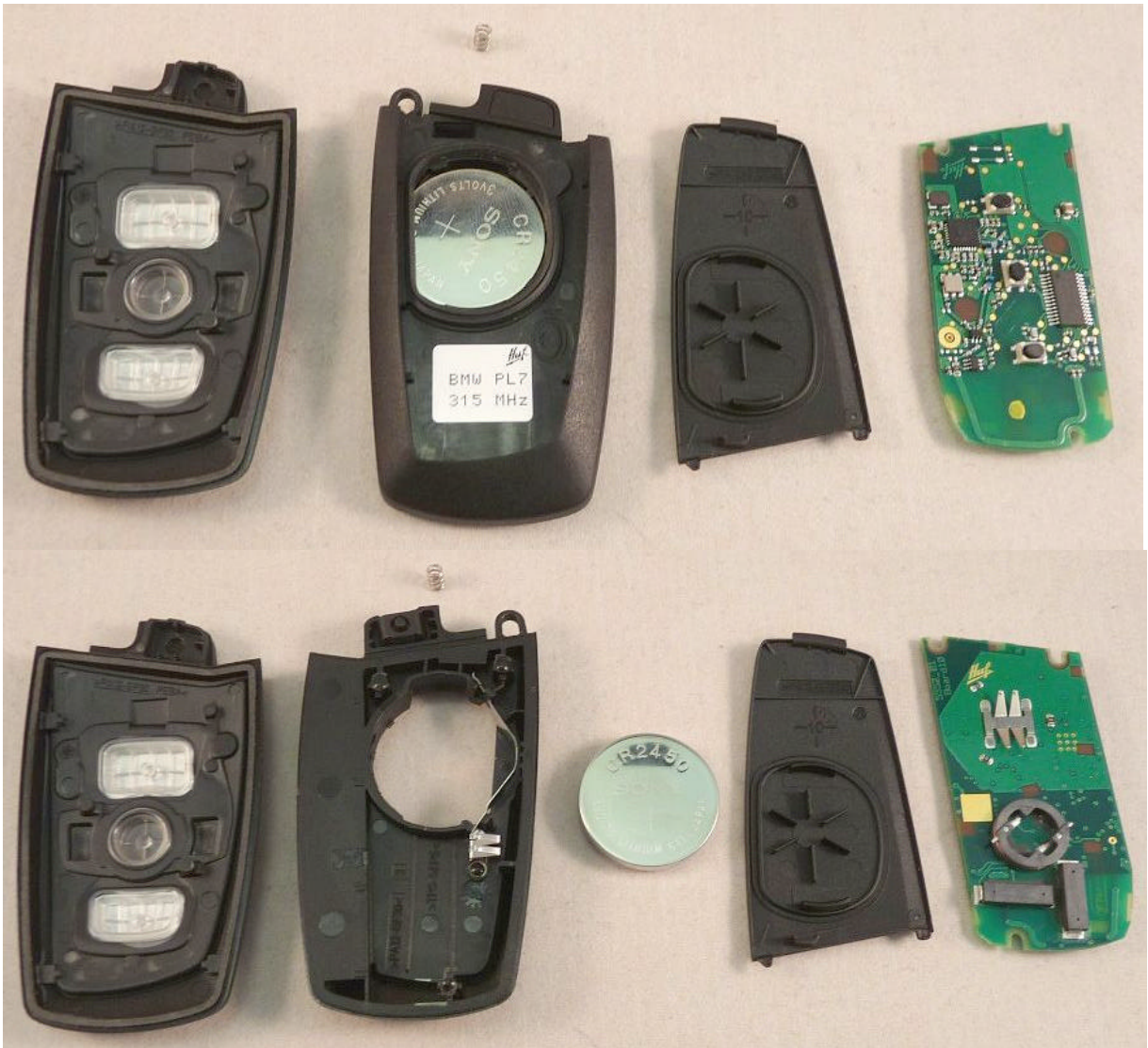
Photos 4: EUT (housing, battery and PCB)
