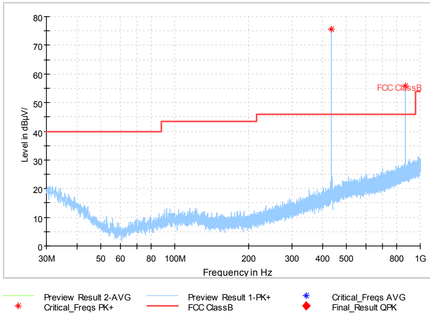
Radiated emission (30MHz – 1GHz)
