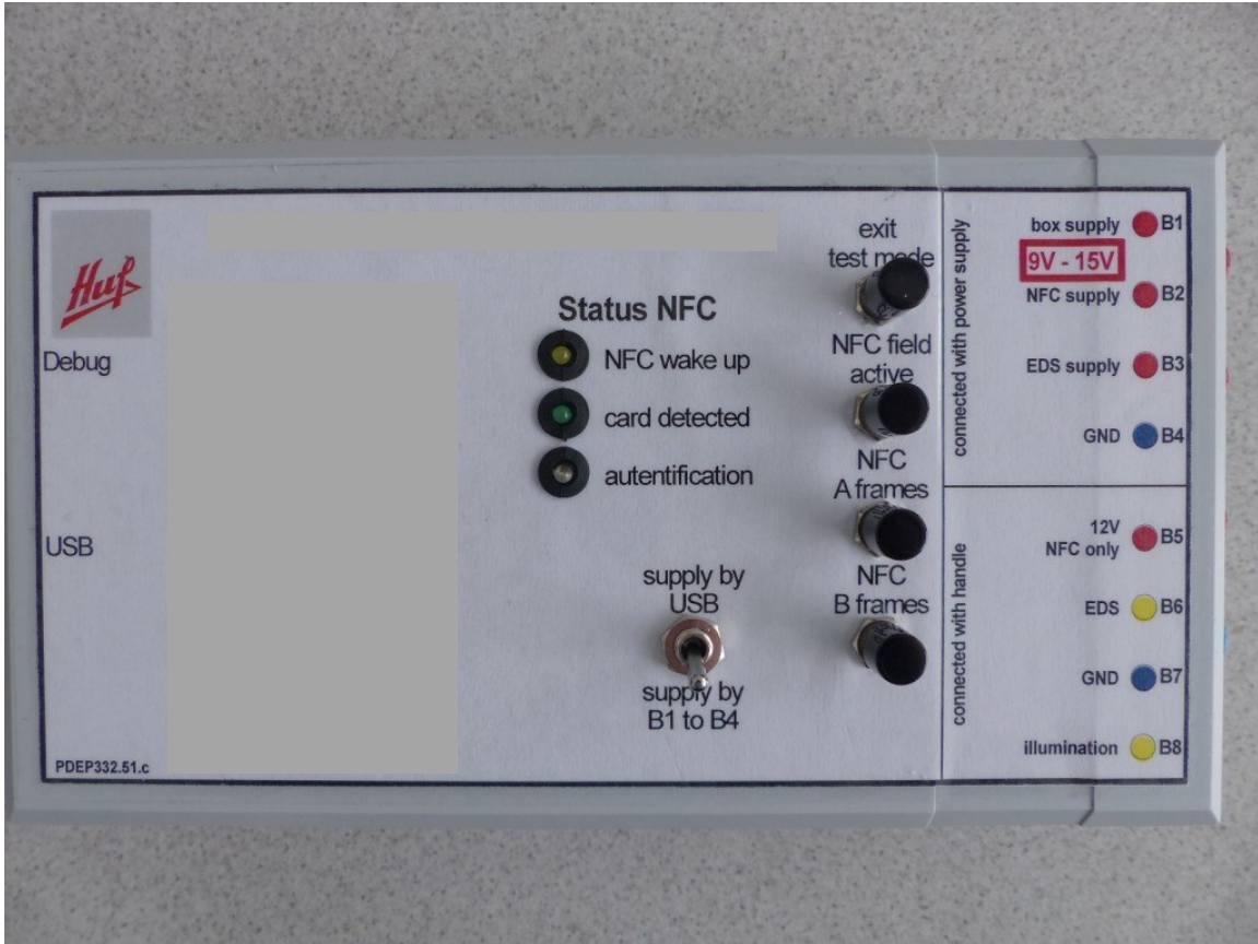
Photo No. 5: Auxiliary Device AUX1
