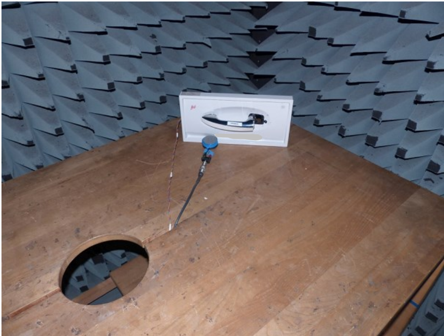
Photo No. 2: Setup for radiated tests ( f < 30 MHz), detailed view
