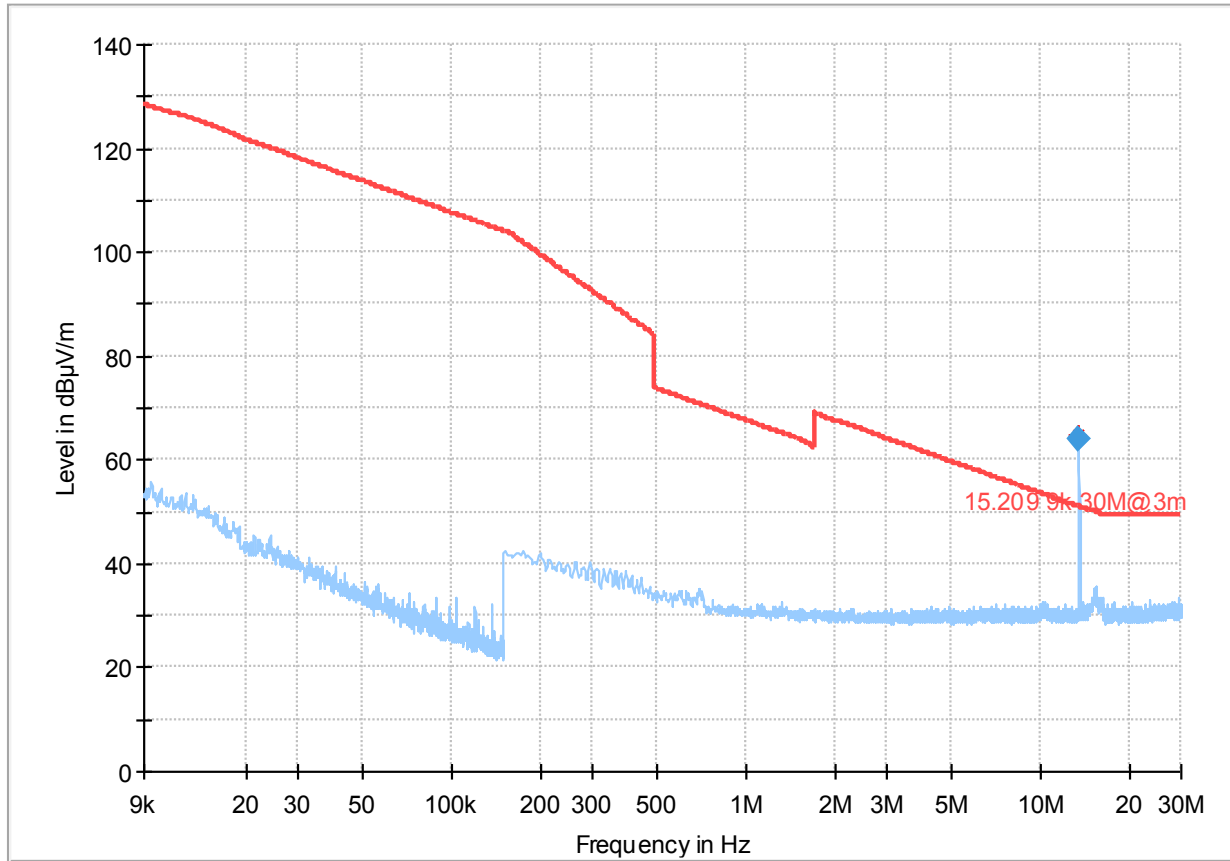
Plot no. 4: Radiated emissions 9 kHz – 30 MHz, Right handle
