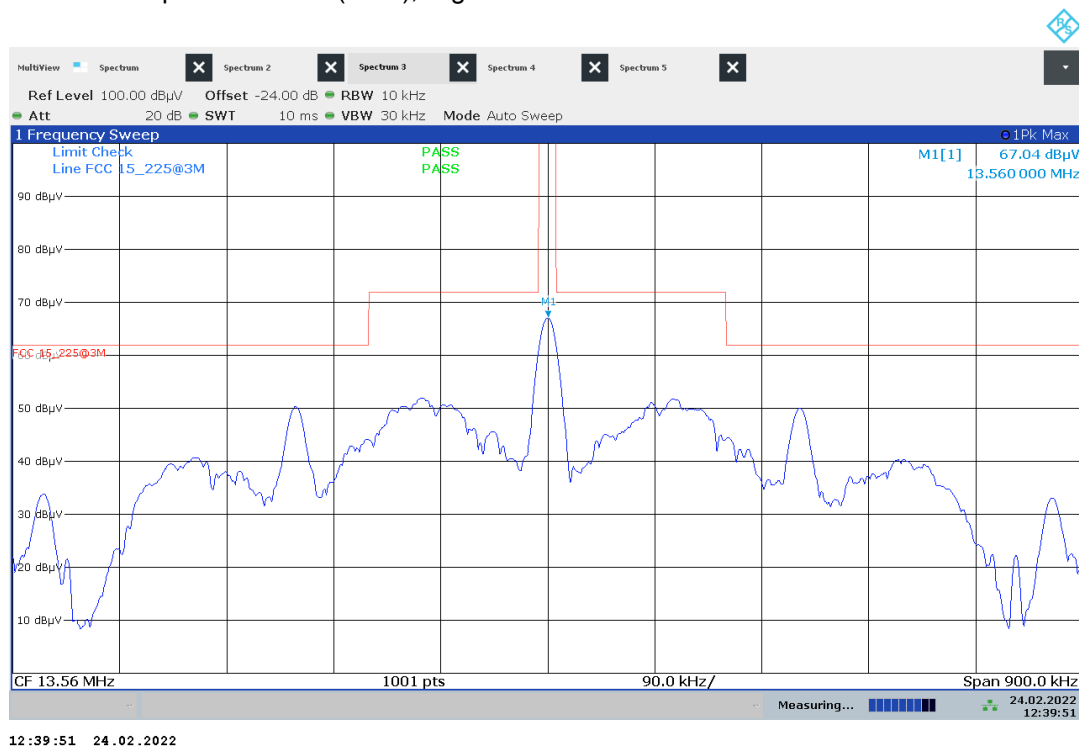
Plot no. 2: Transmitter Spectrum Mask (TSM), Right handle
