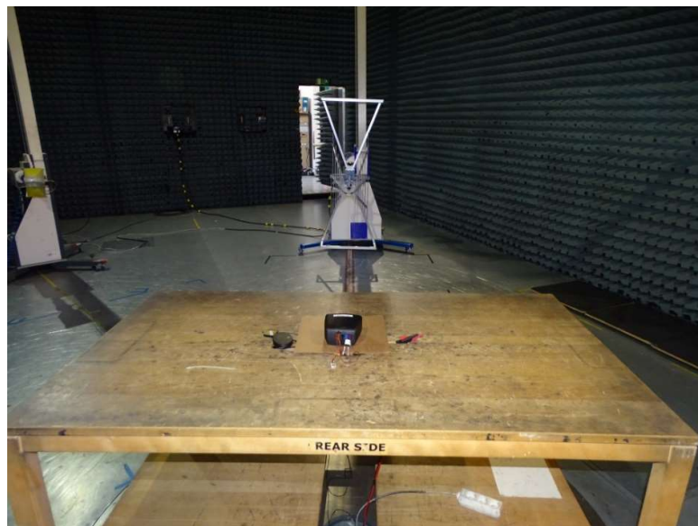
Photo 2: Test setup for radiated emissions measurements in semi-anechoic chamber (30 MHz to 1 GHz), front side view
