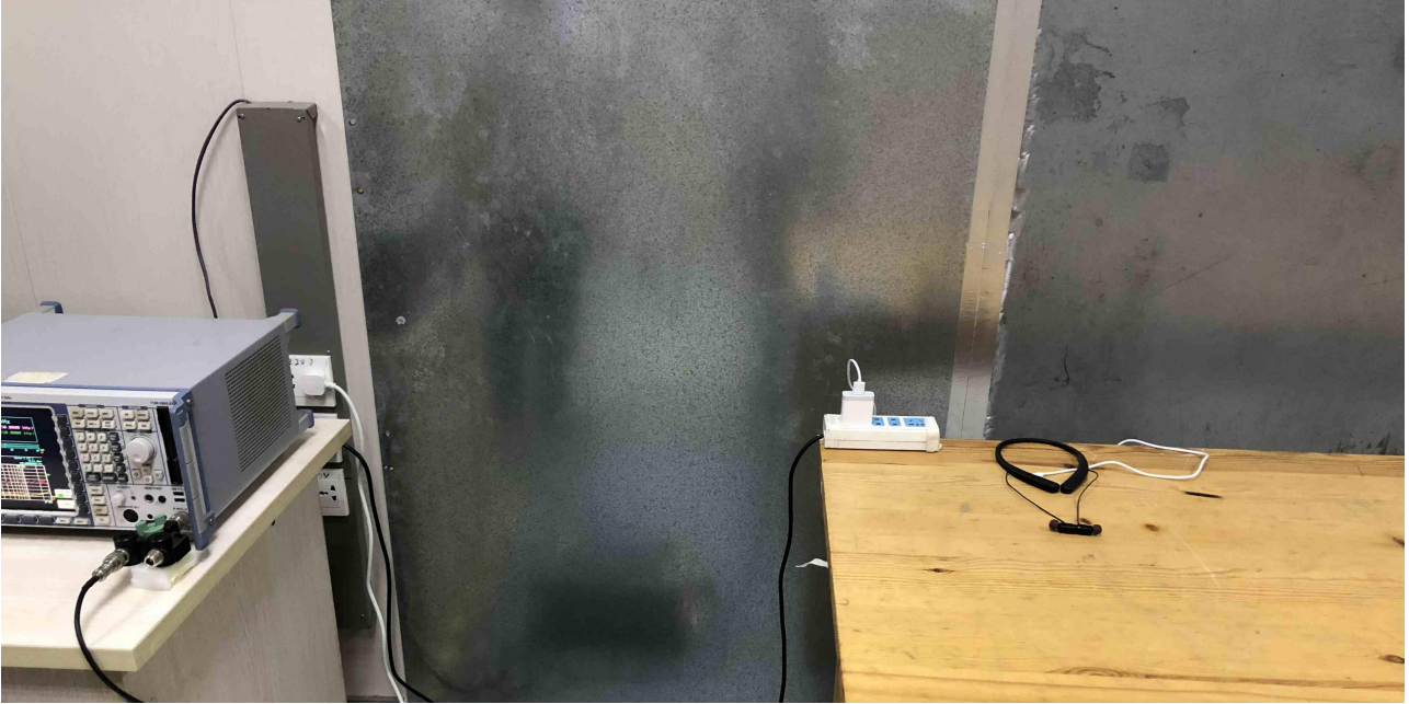
Radiated Spurious Emissions Test Frequency From 30MHz-1000MHz
