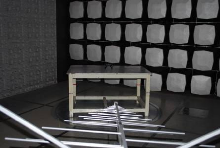
Radiated Emission
