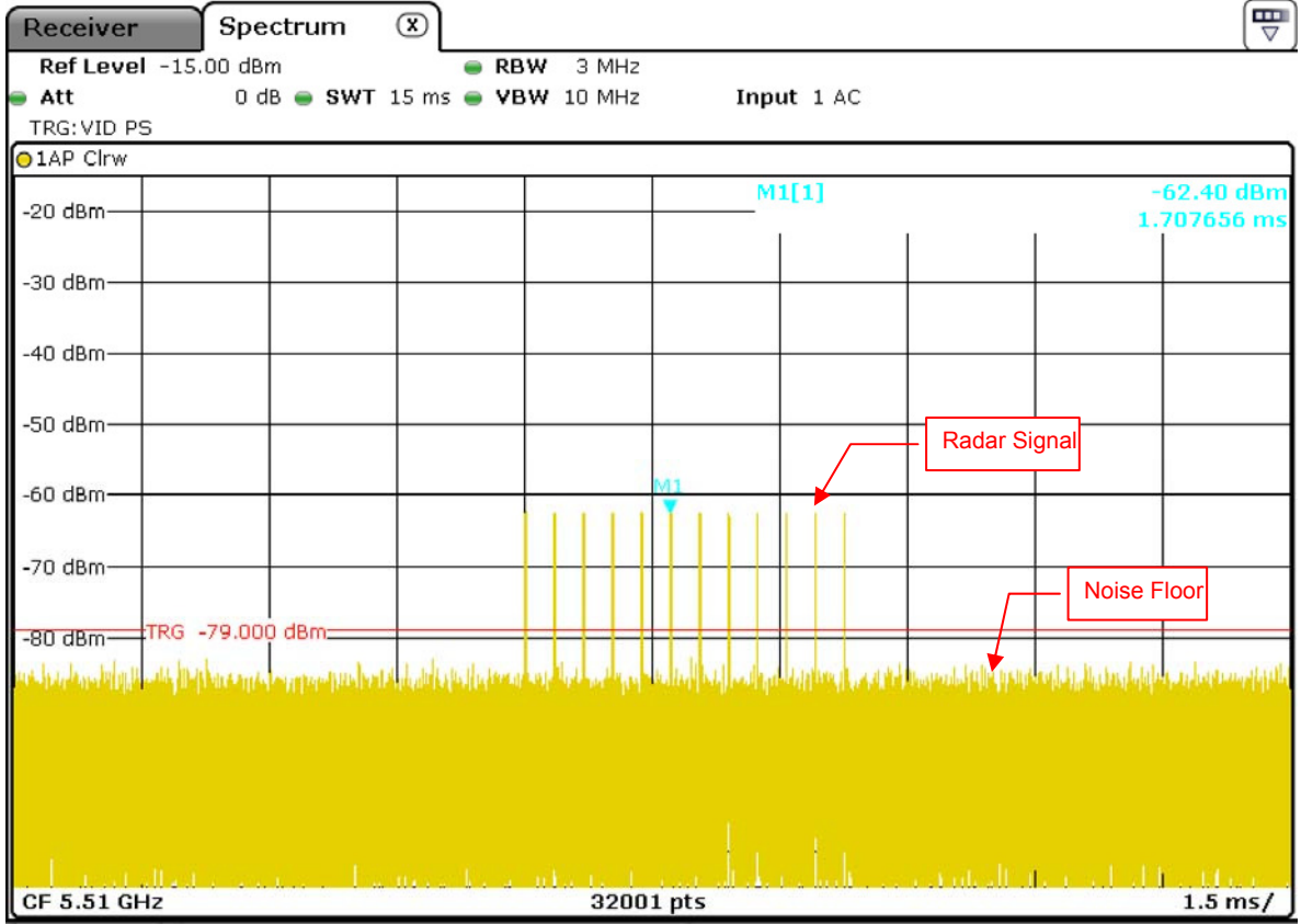
Radar Signal 4
