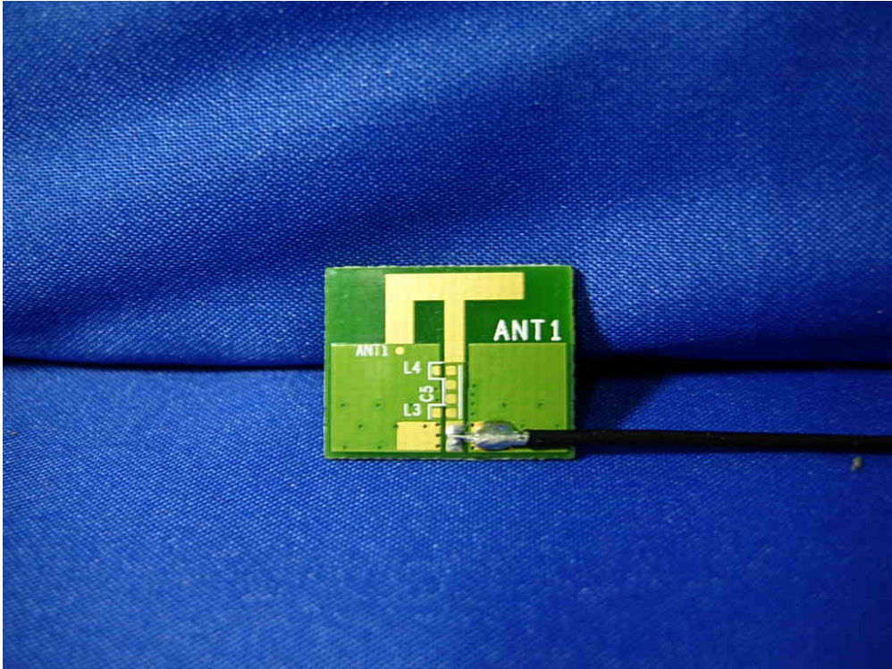
(19) EUT Photo (External Antenna)
