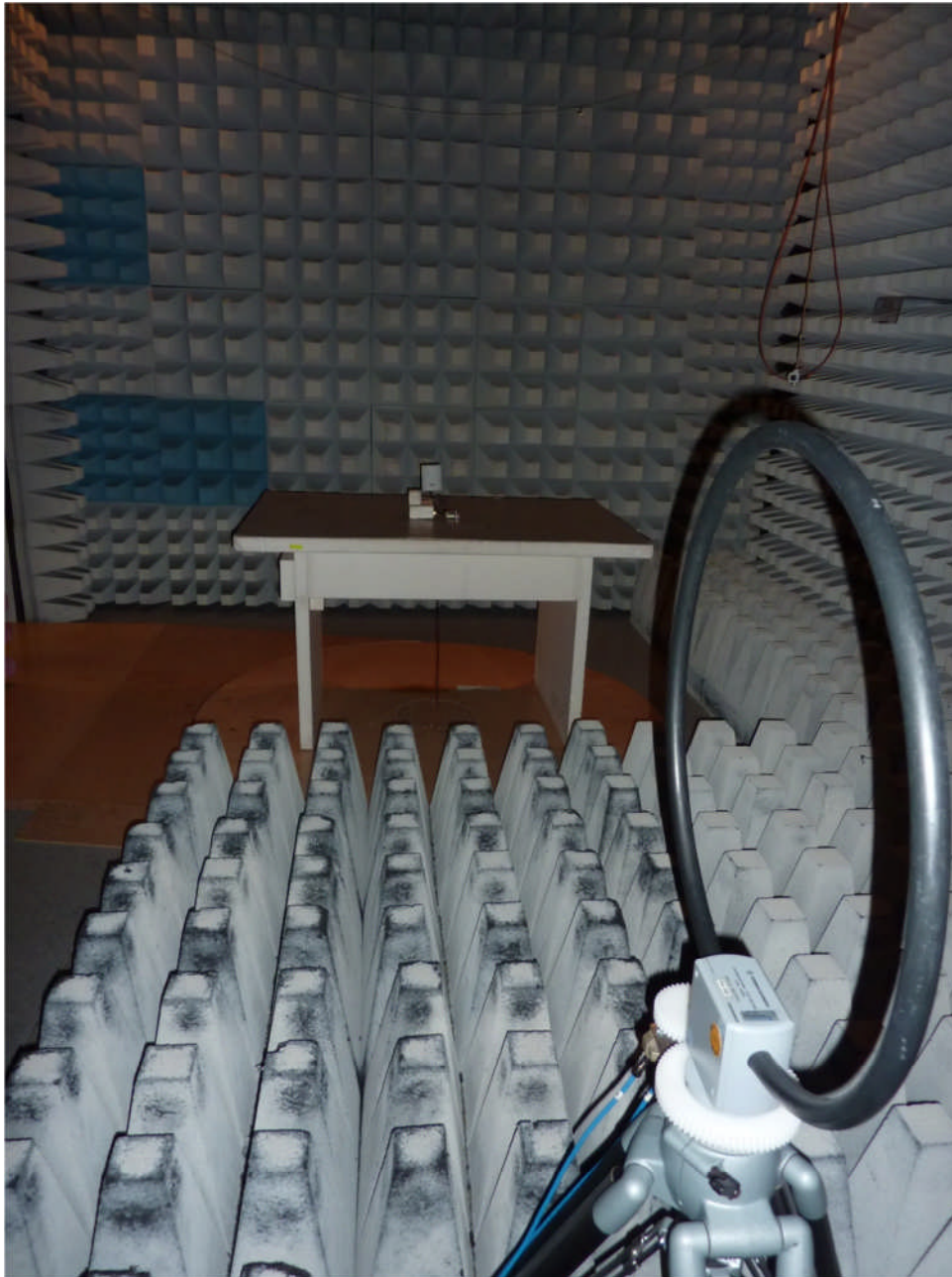
114368_11: Test setup fully anechoic chamber (patch antenna)
