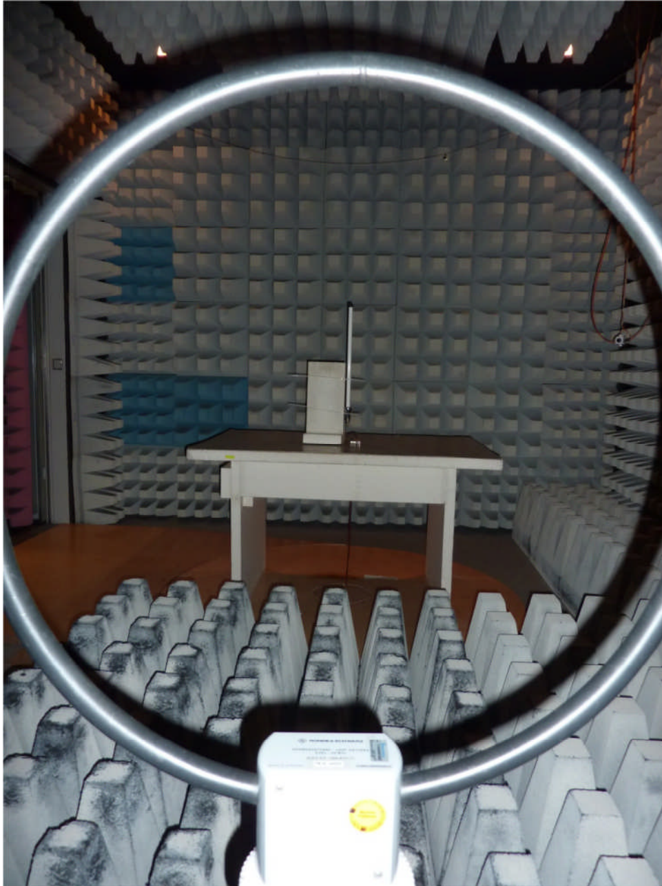
114368_10: Test setup fully anechoic chamber (monopole antenna)
