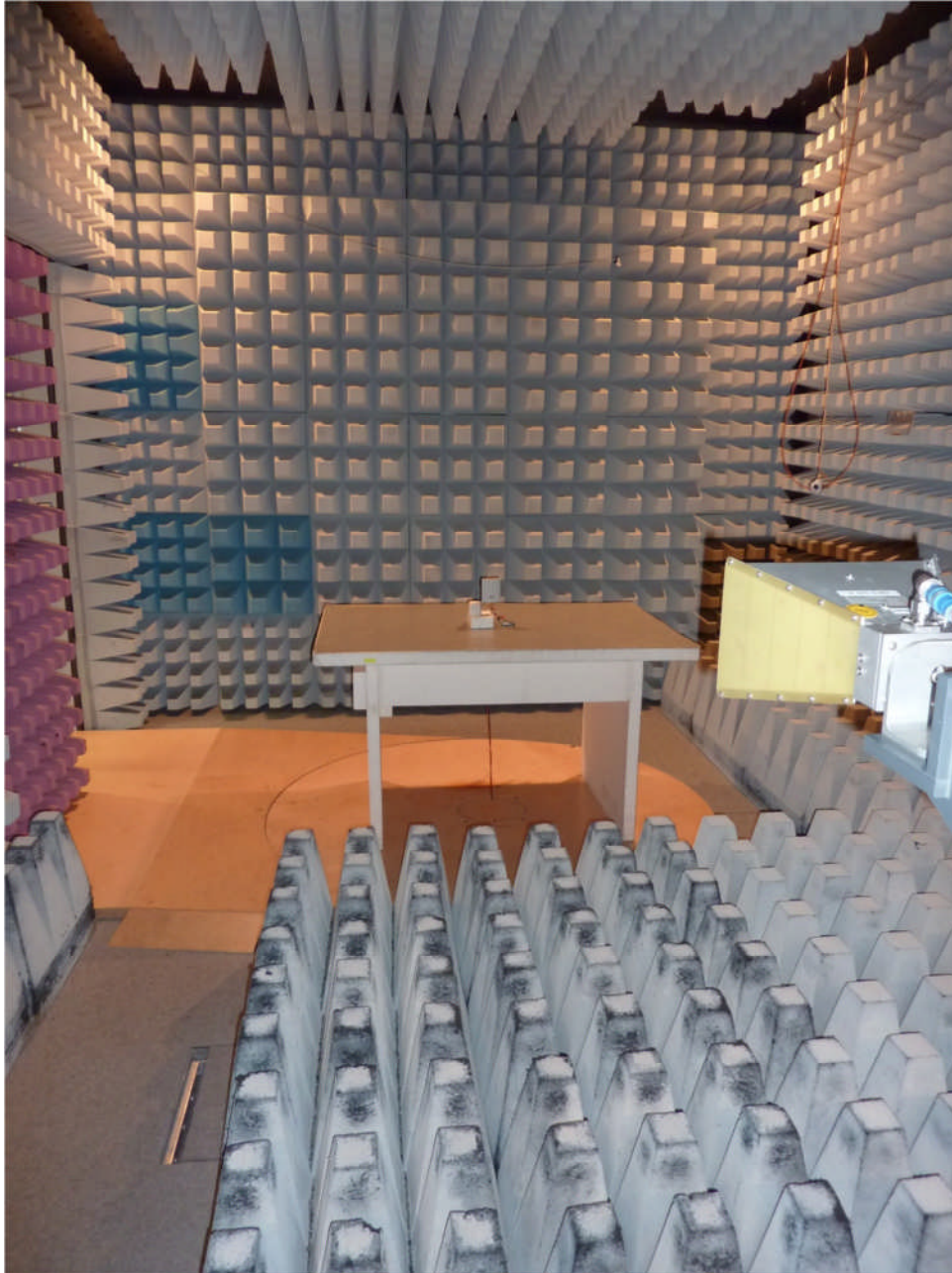
114368_03: Test setup fully anechoic chamber (patch antenna)
