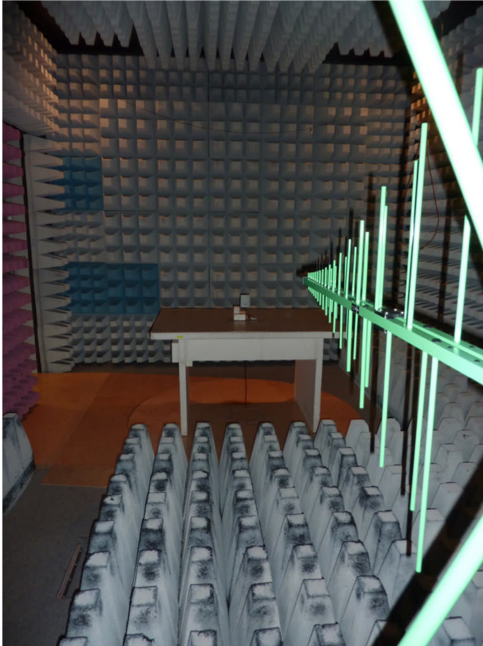
114368_09: Test setup fully anechoic chamber (patch antenna)
