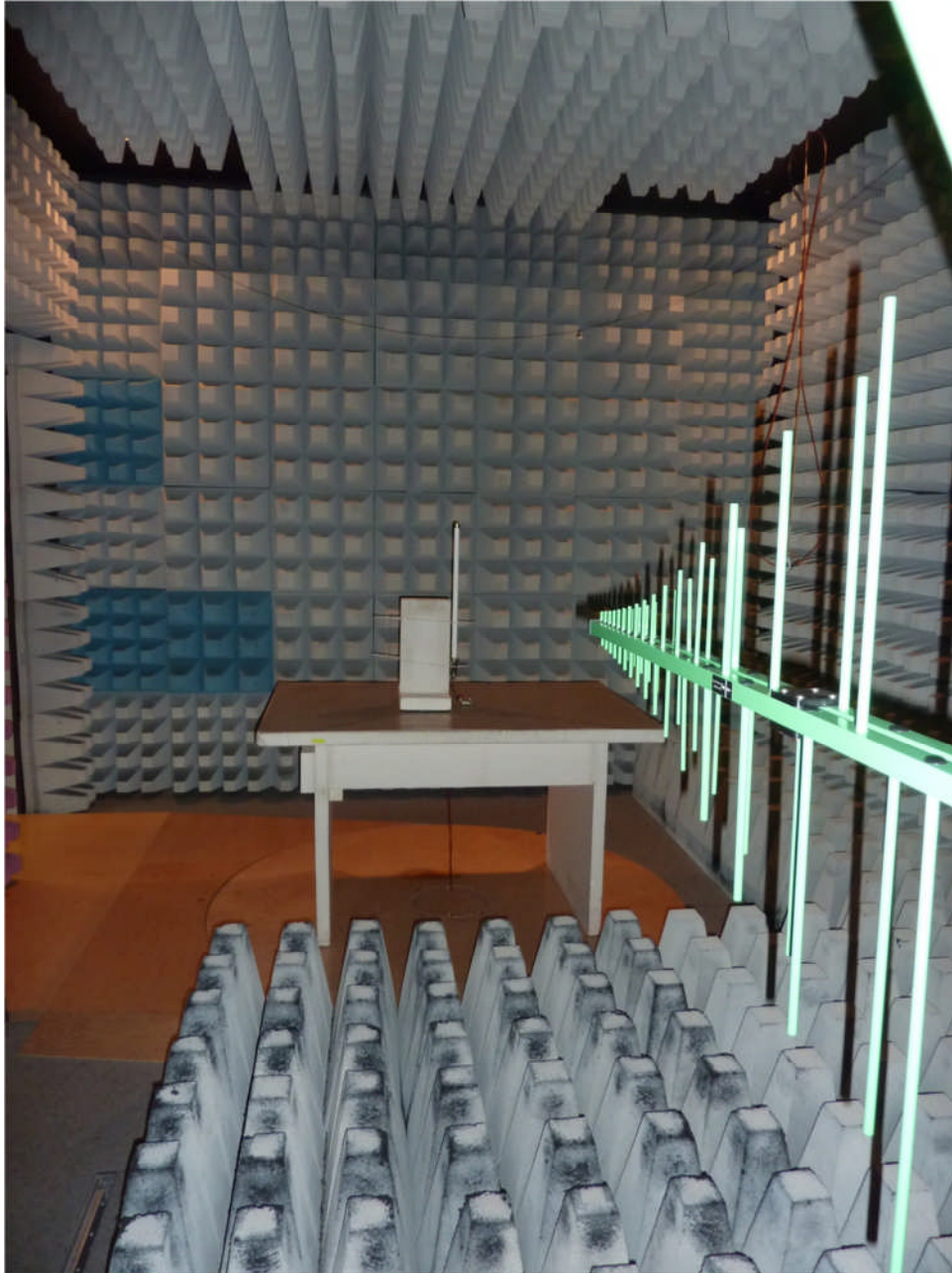
114368_08: Test setup fully anechoic chamber (monopole antenna)
