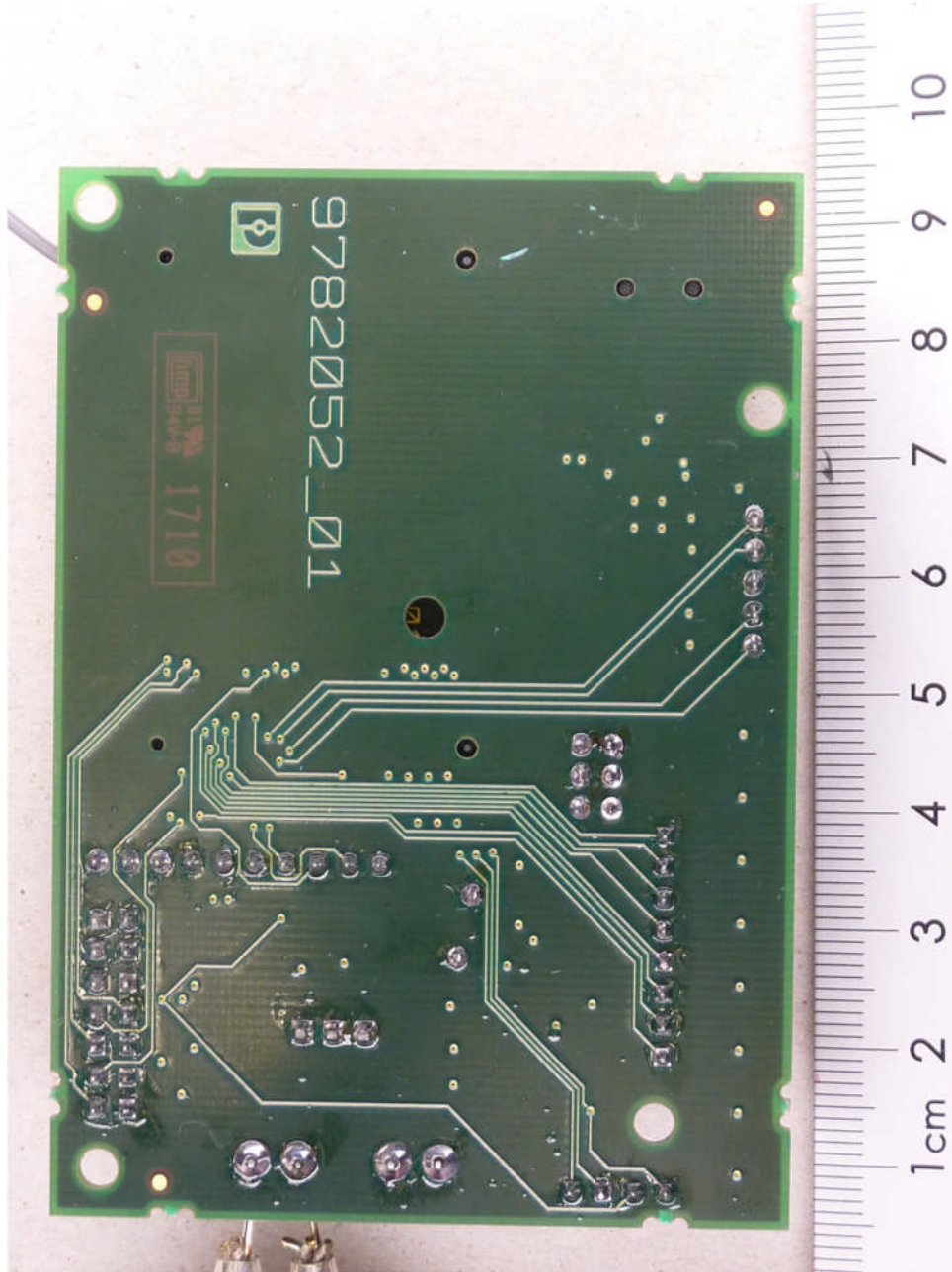
114368_EUT02: Carrier board, rear view
