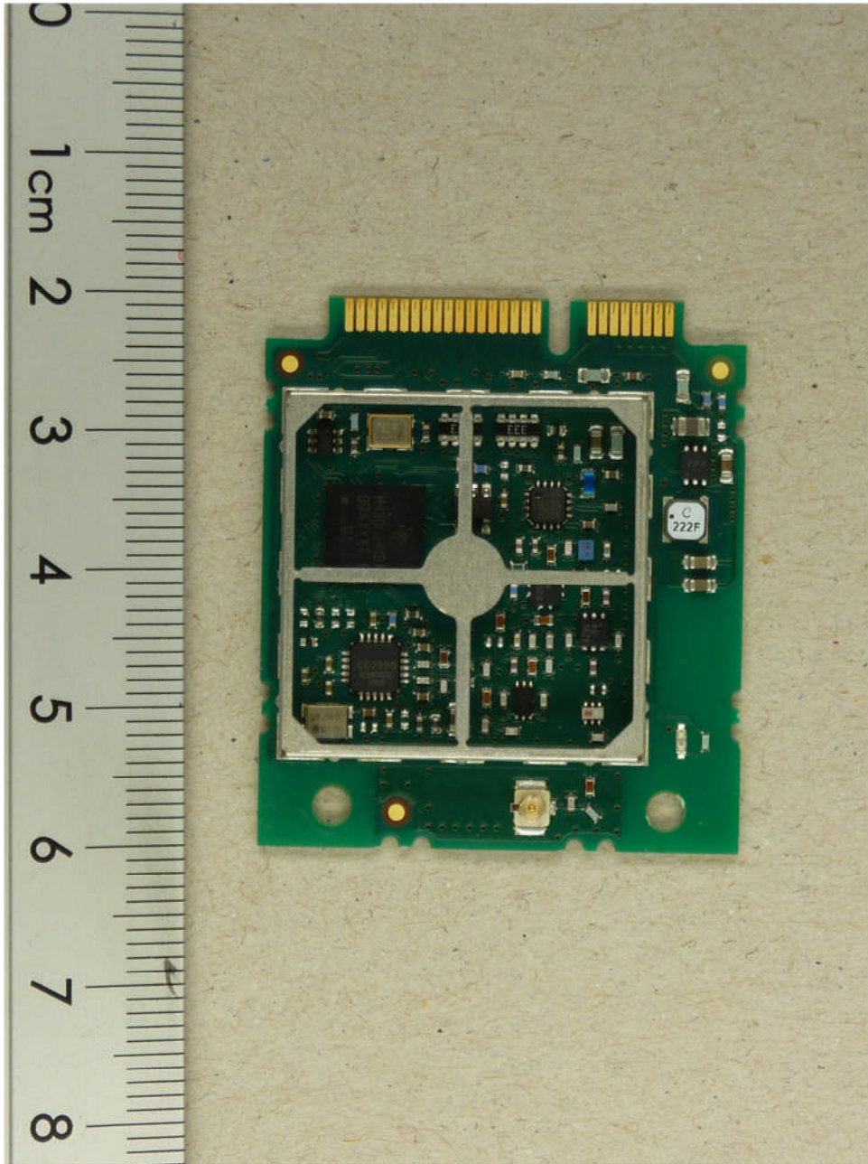
114368_EUT05: SiWiNet, top view (shielding removed)
