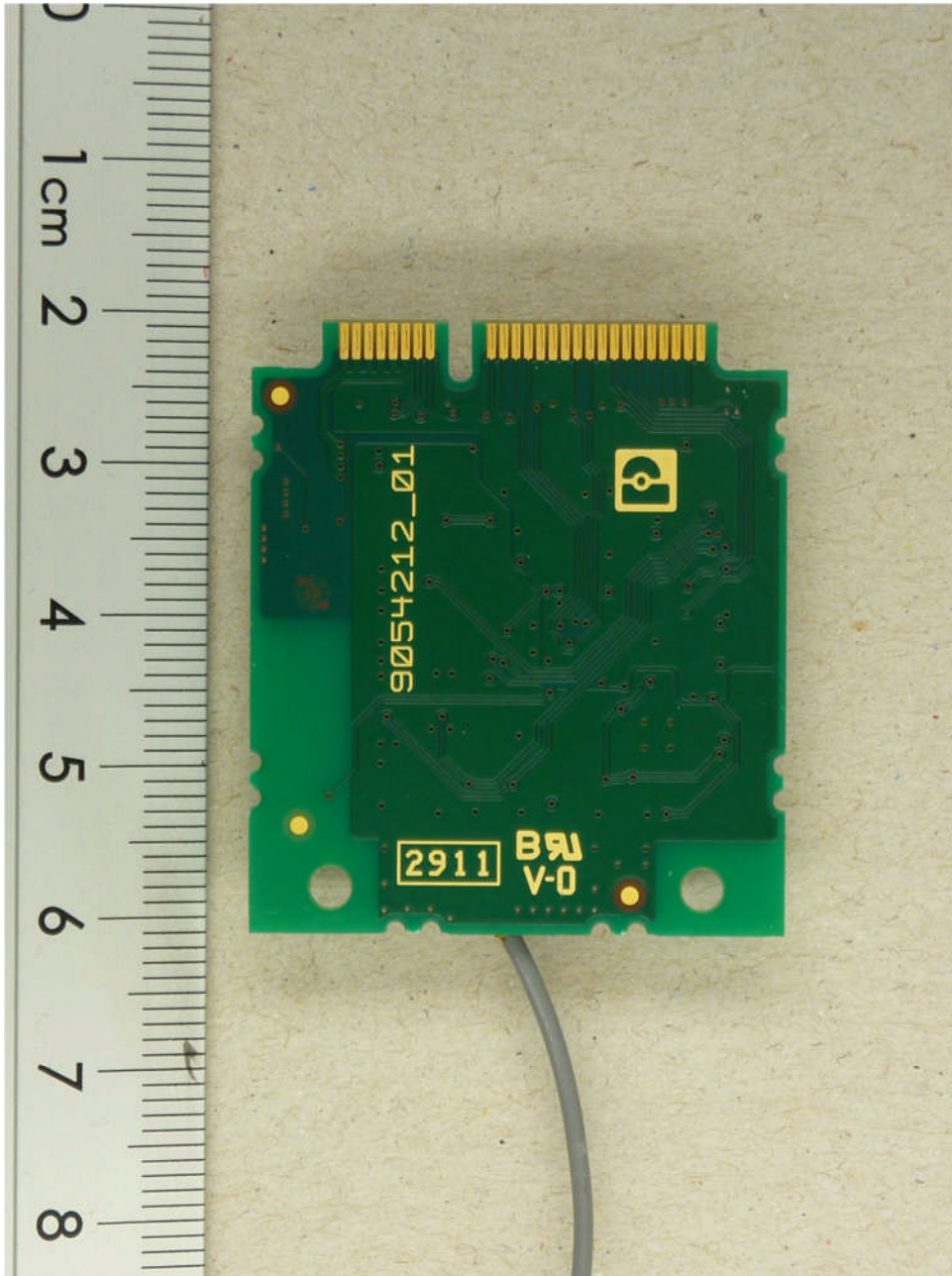
114368_EUT04: SiWiNet, bottom view
