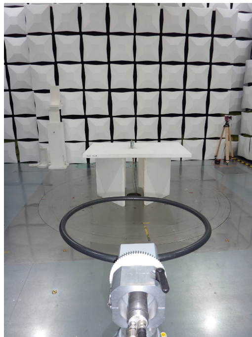
Test setup - Radiated emission (semi anechoic chamber) 9 kHz – 30 MHz
