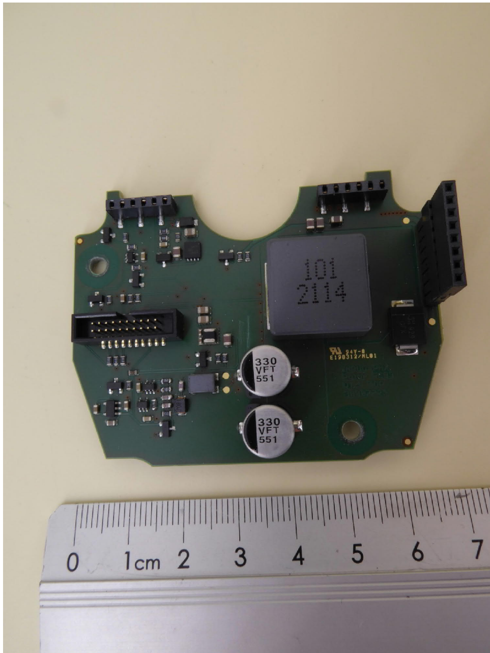
NEARFI PD 2A ETH R, energy PCB, top view
