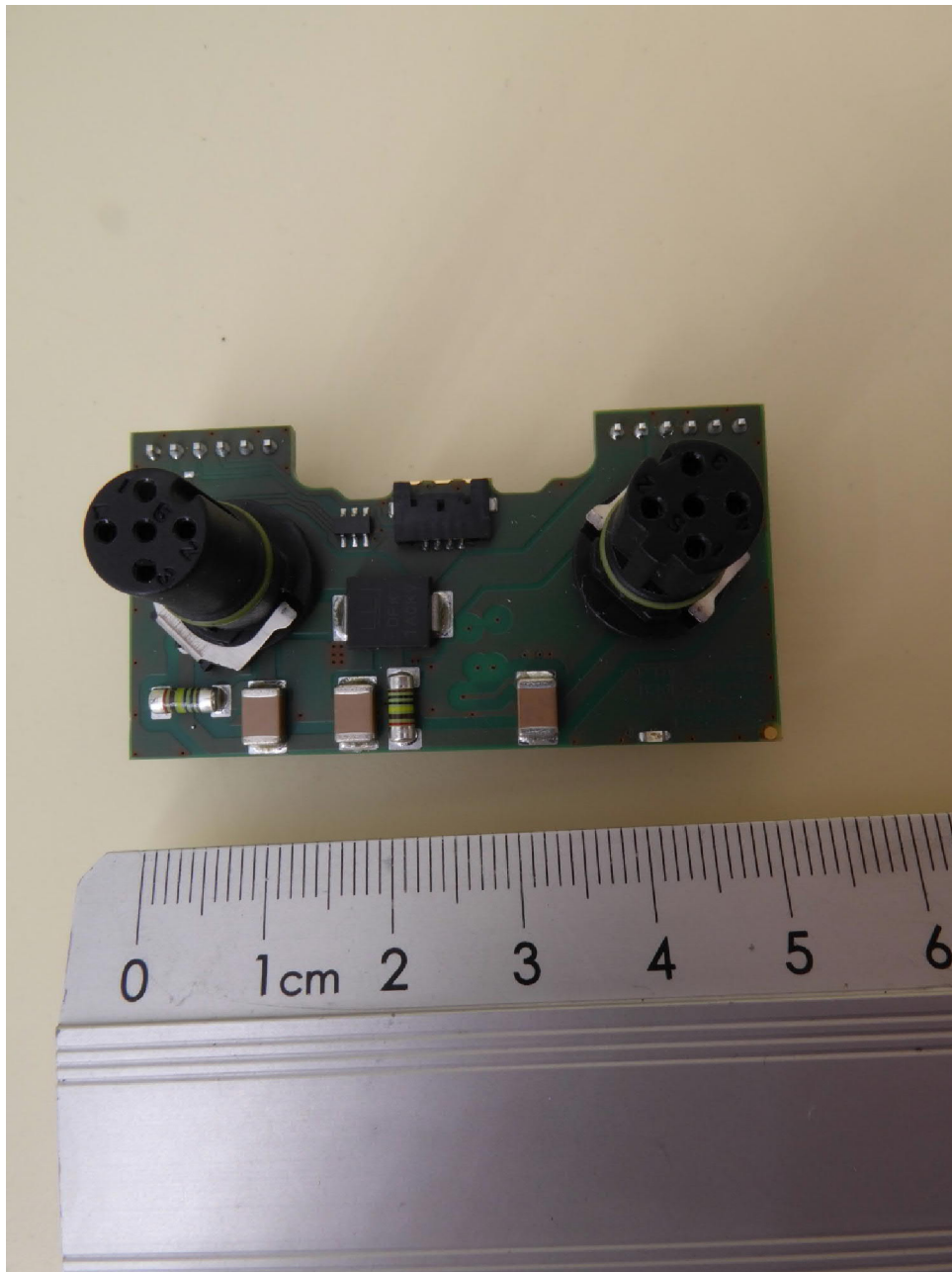
NEARFI PD 2A ETH R, interface PCB, top view
