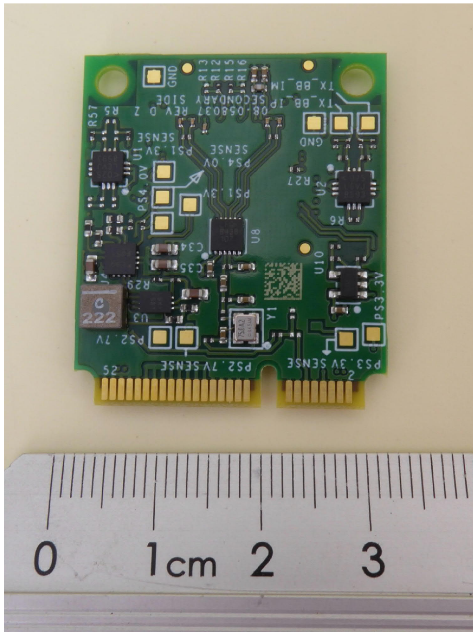
NEARFI PD 2A ETH R, RF-PCB, bottom view
