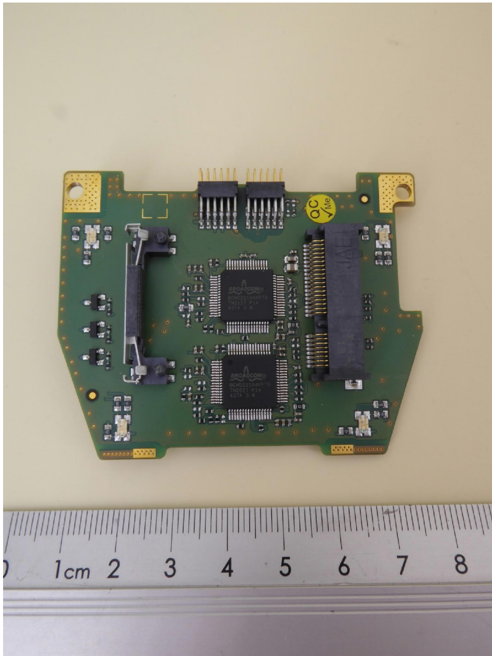
NEARFI PD 2A ETH R, data PCB, top view
