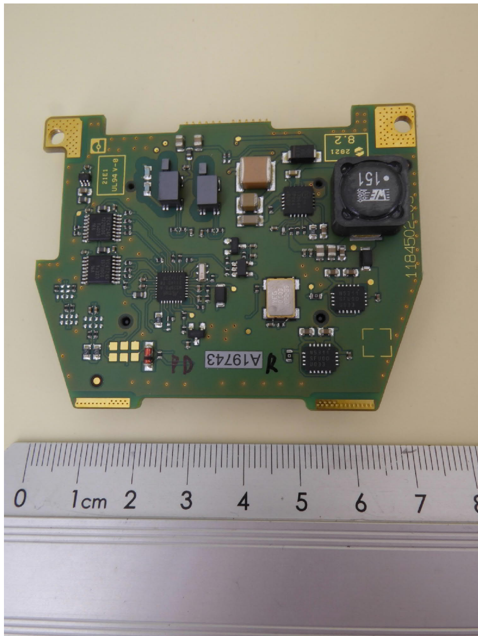
NEARFI PD 2A ETH R, data PCB, bottom view
