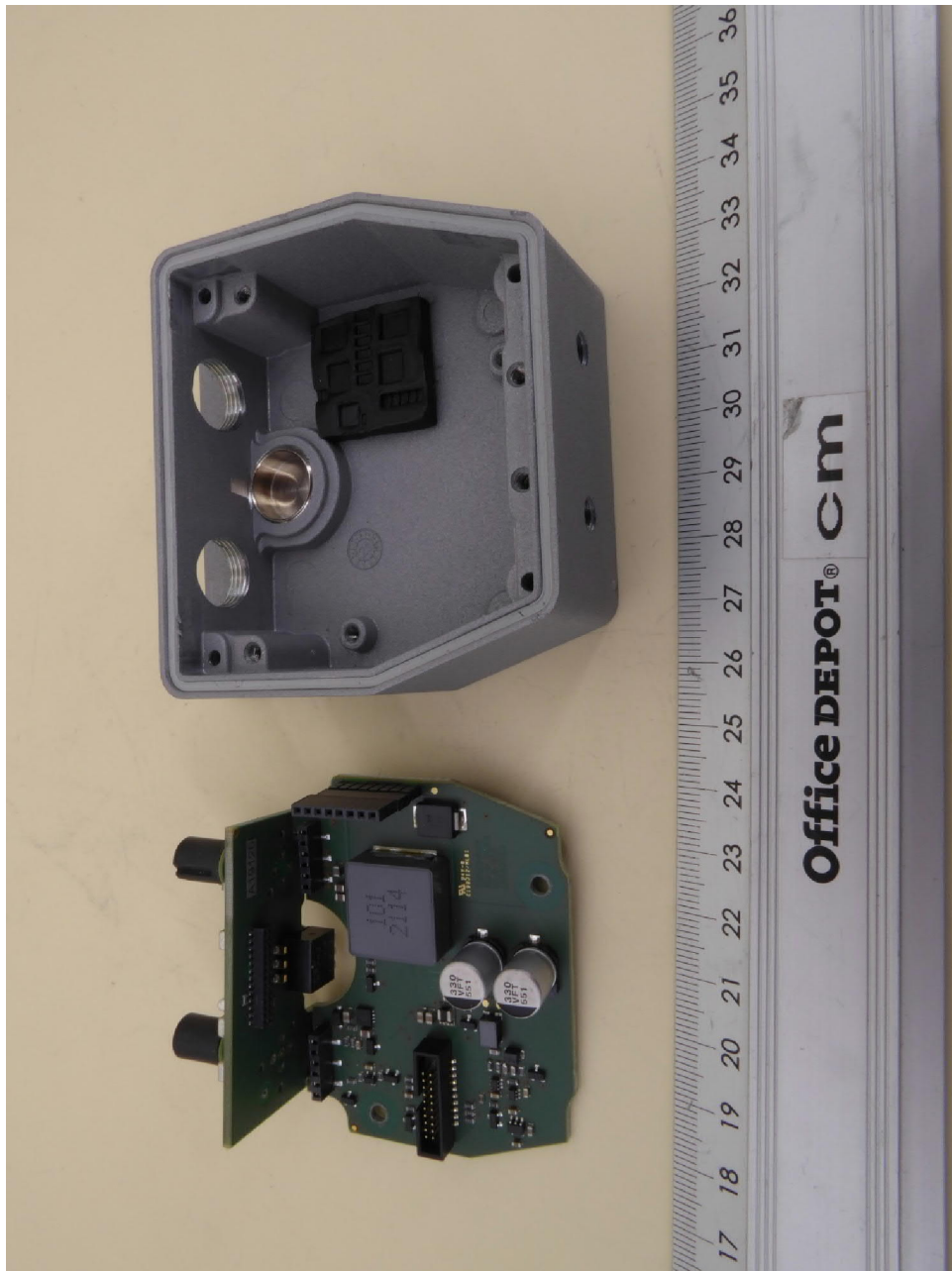
NEARFI PD 2A ETH R, internal view 5, energy PCB removed
