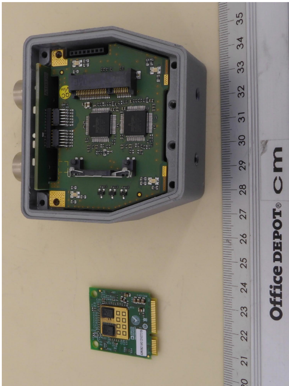
NEARFI PD 2A ETH R, internal view 3, RF-PCB removed
