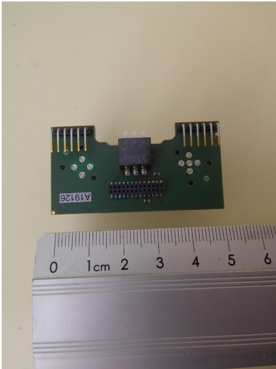
NEARFI PD 2A ETH R, interface PCB, bottom view
