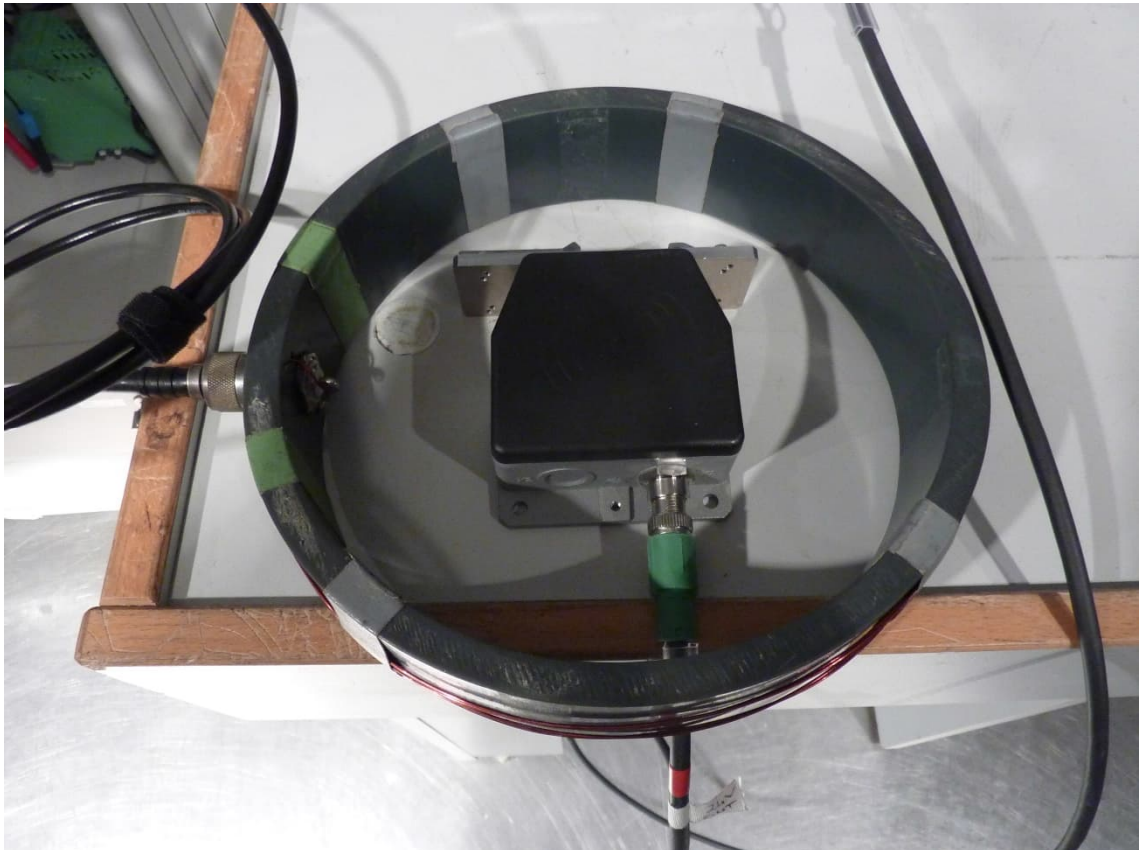
Test setup - Radiated emission (Test fixture)
