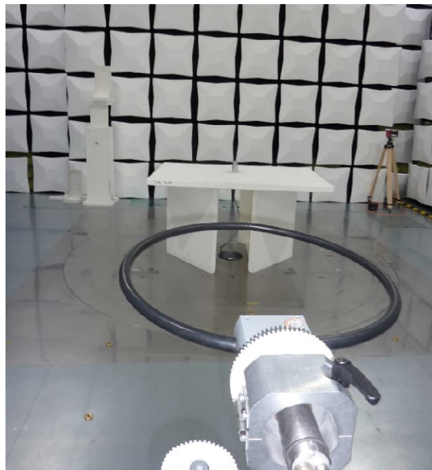
Test setup - Radiated emission (semi anechoic chamber) 9 kHz – 30 MHz
