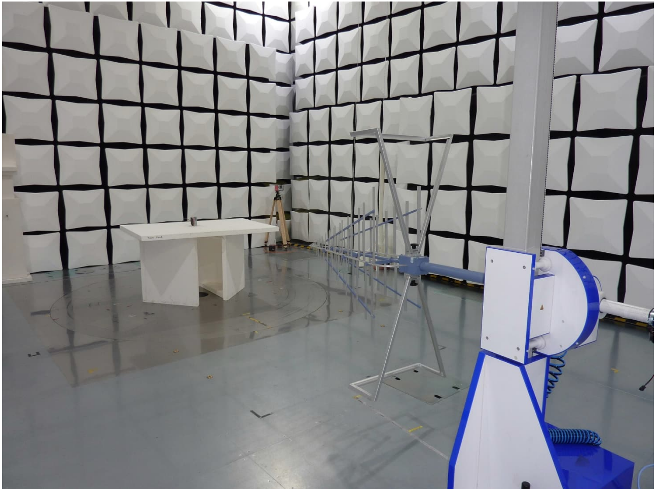
Test setup - Radiated emission (semi anechoic chamber) 30 MHz – 1000 MHz
