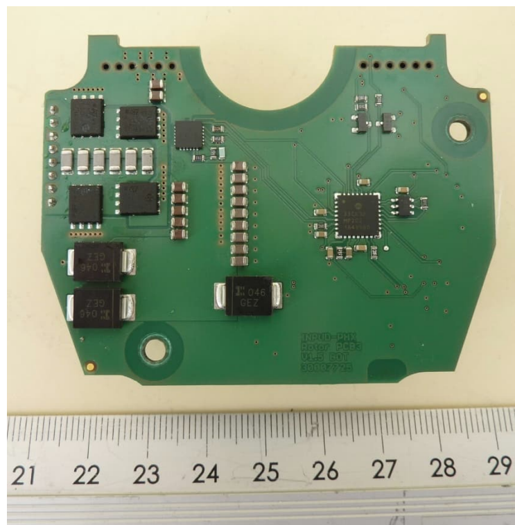
EUT (Base) – Energy PCB
