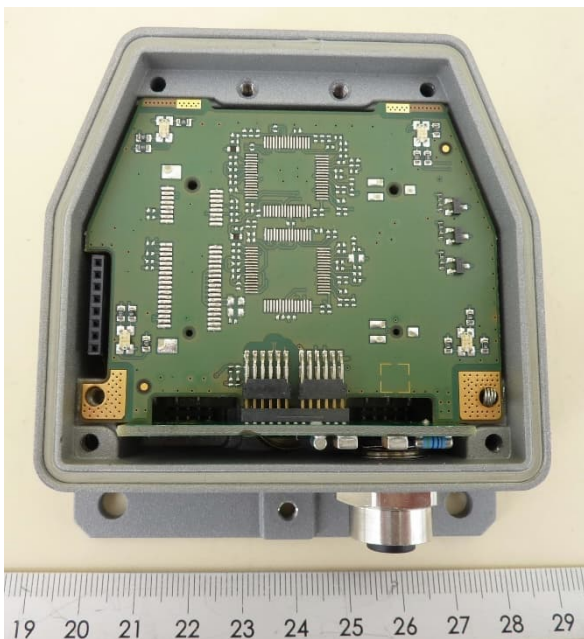
EUT (Base) – Cabinet opened
