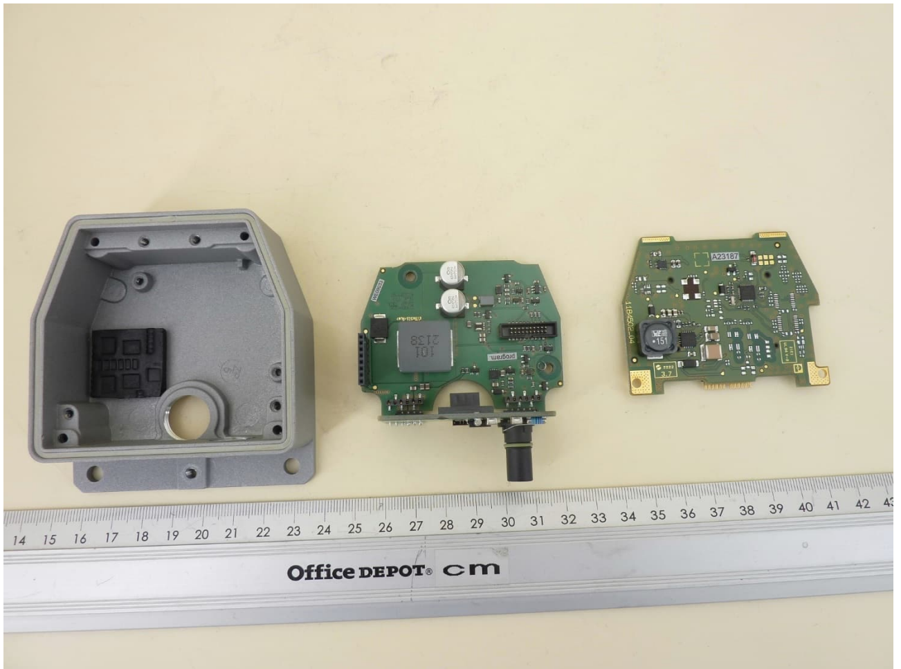
EUT (Base) – Cabinet opened
