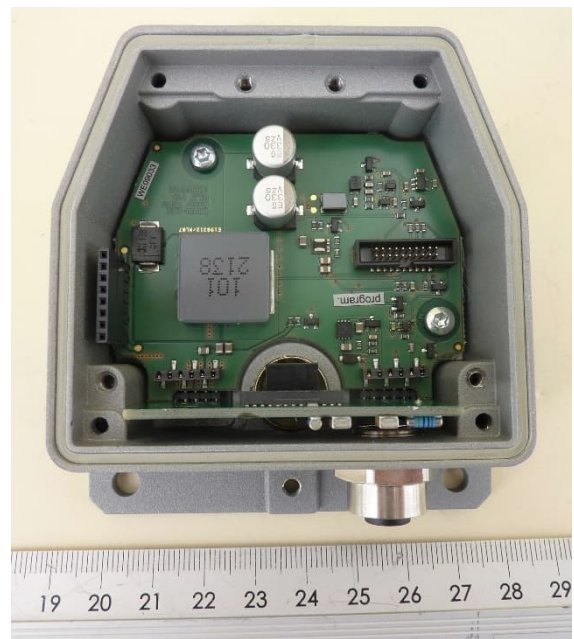
EUT (Base) – Cabinet opened
