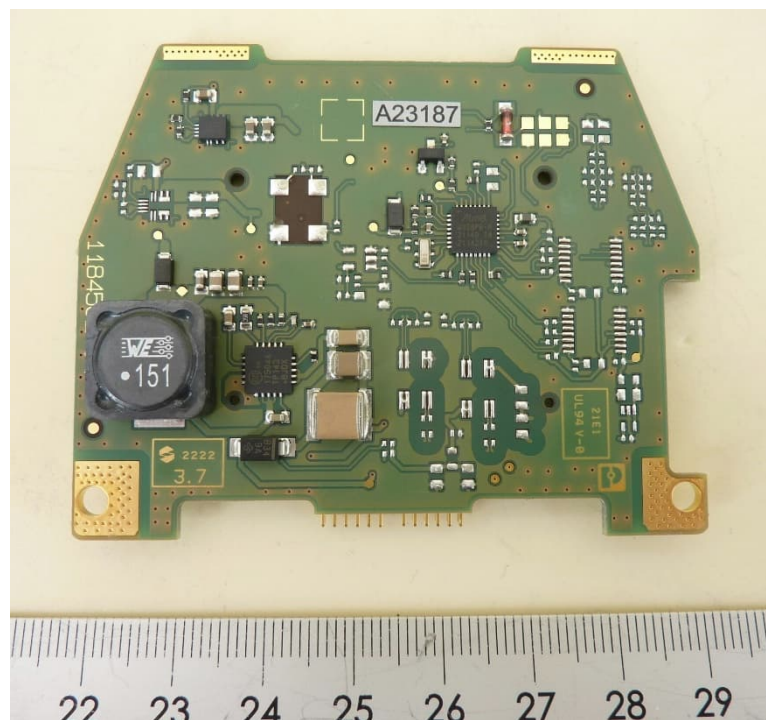
EUT (Base) – Data PCB
