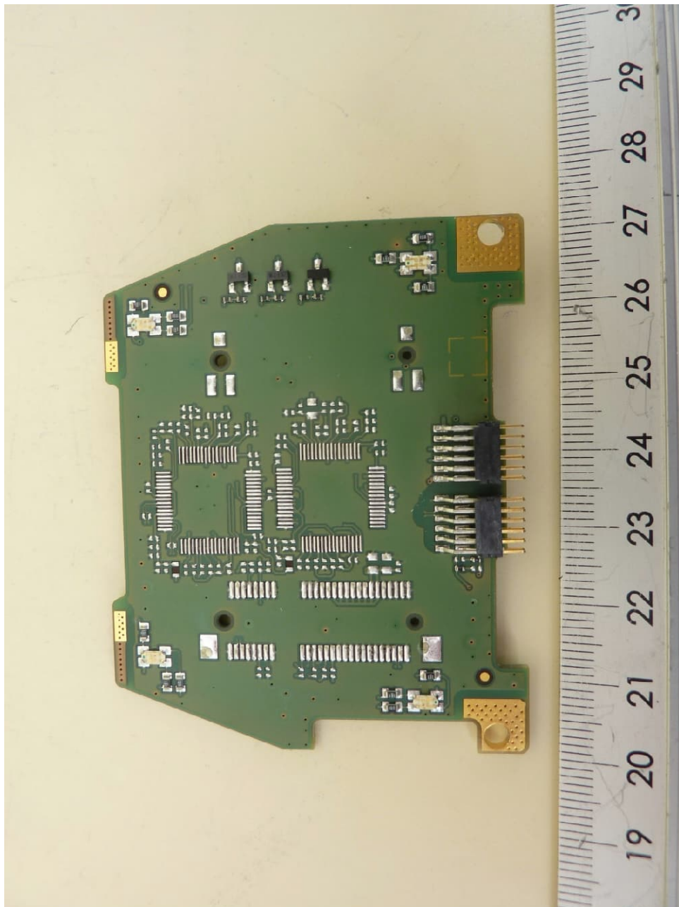
NEARFI P 2A B, data PCB, top view
