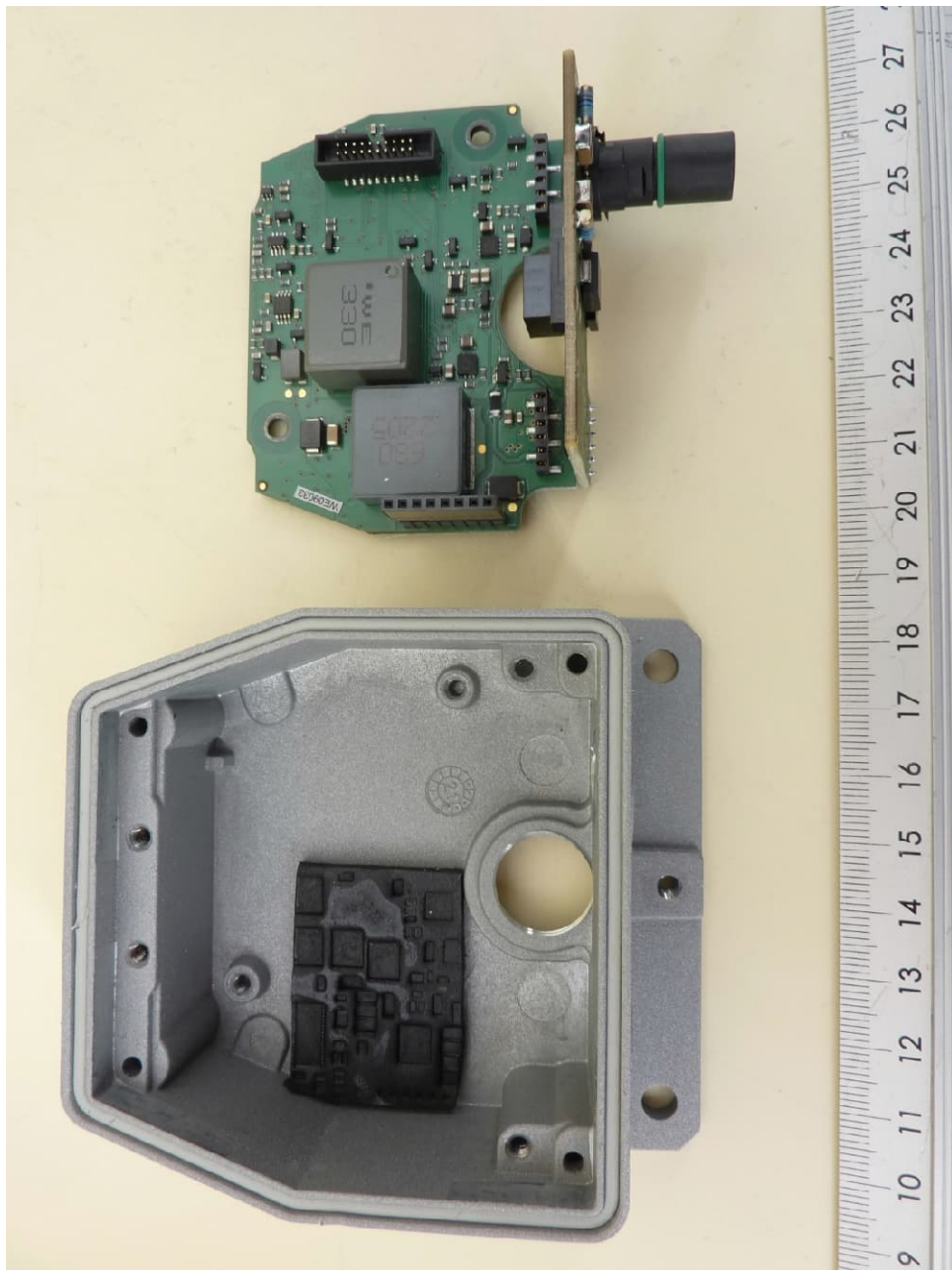
NEARFI P 2A B, internal view 4, energy PCB removed
