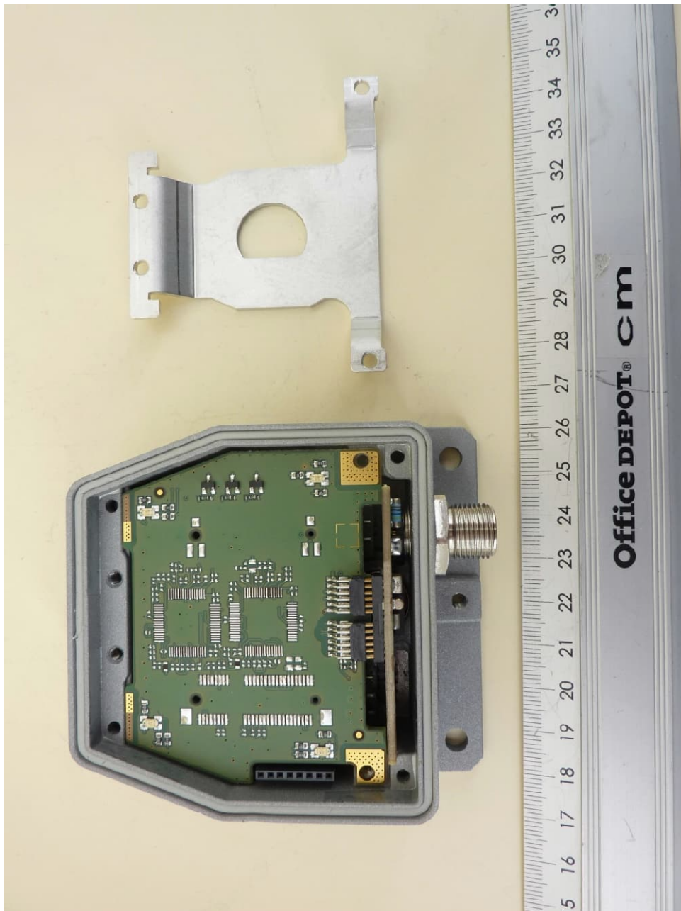
NEARFI P 2A B, internal view 2, shielding removed
