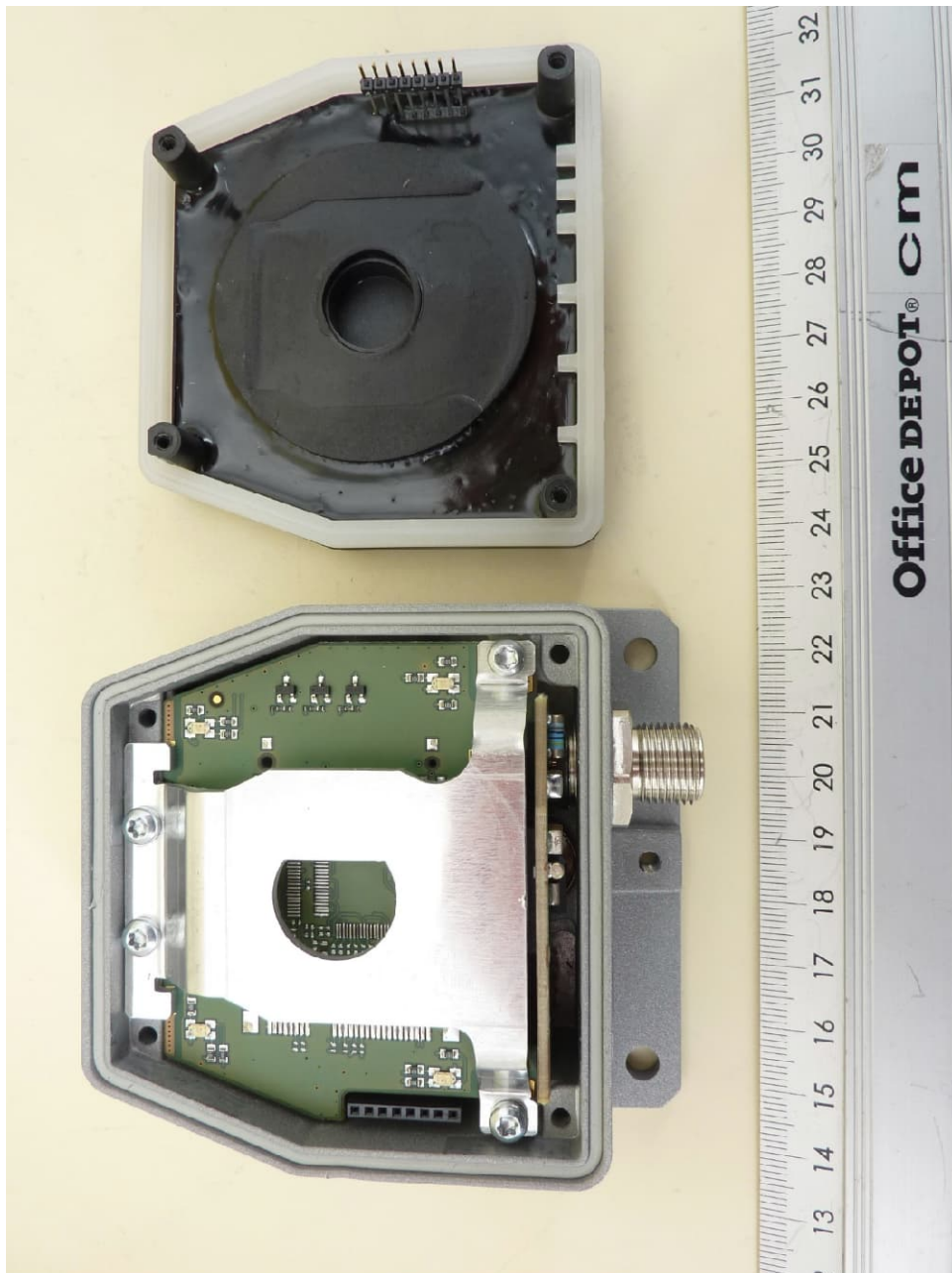
NEARFI P 2A B, internal view 1, housing opened
