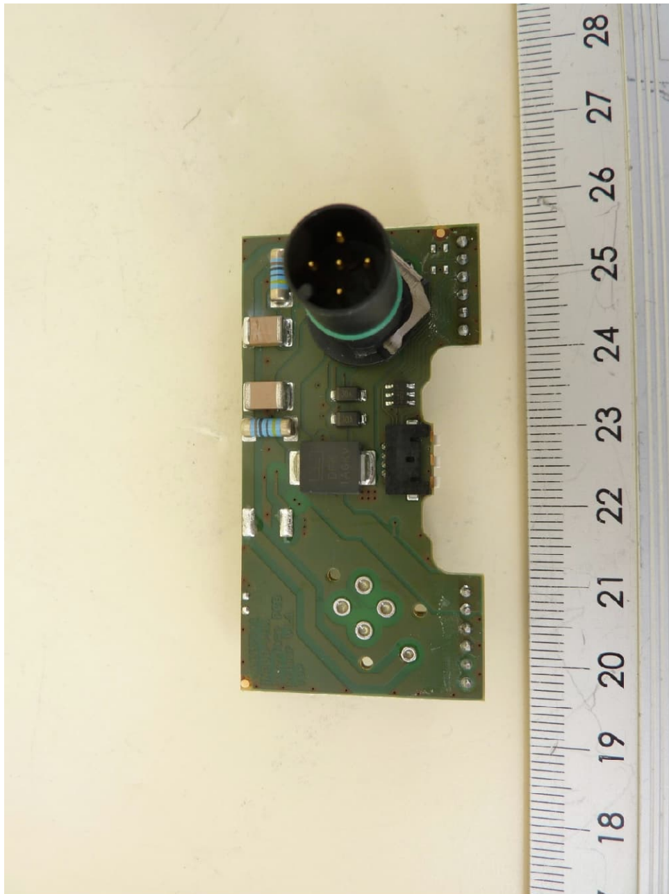
NEARFI P 2A B, interface PCB, top view
