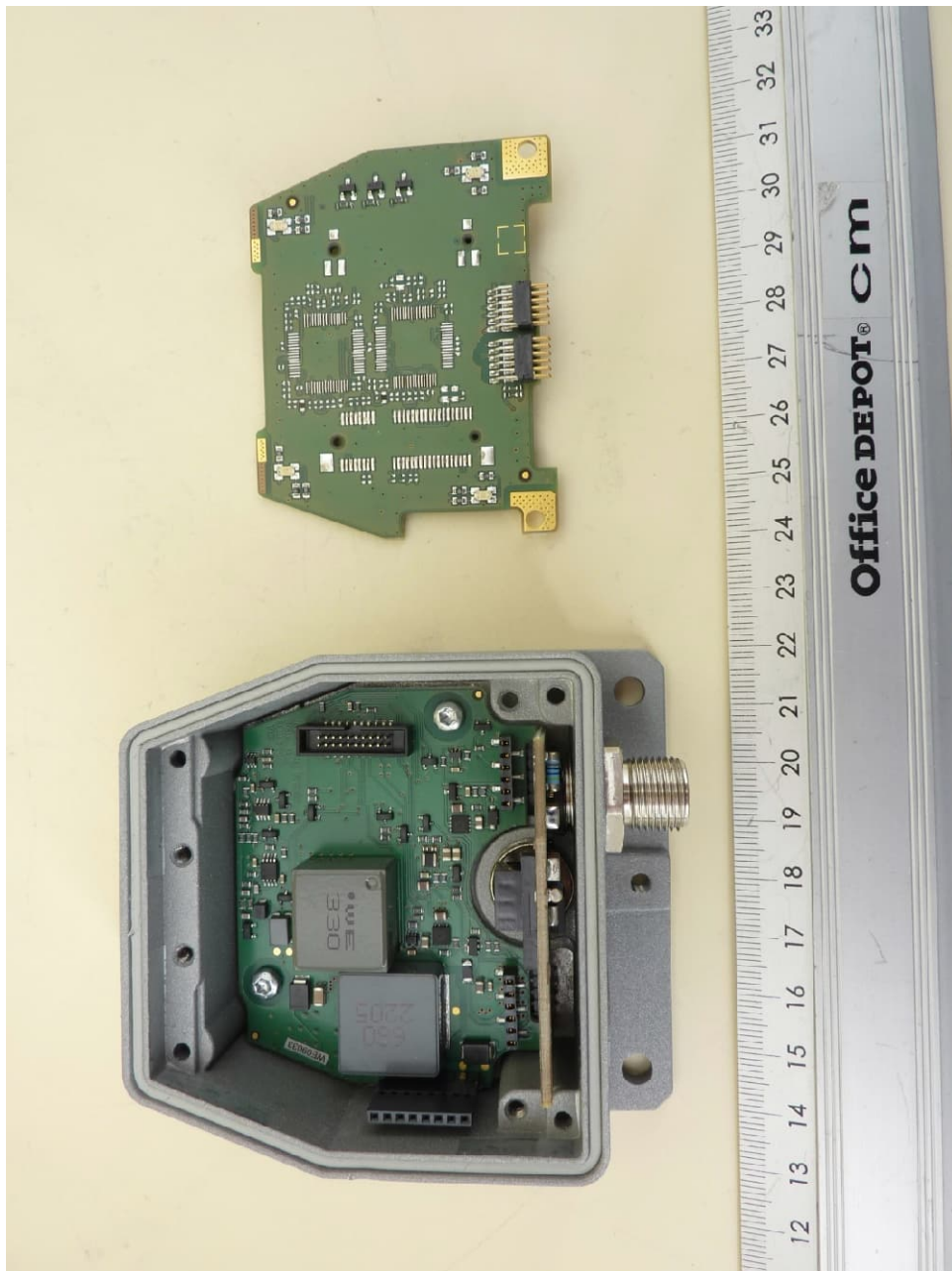
NEARFI P 2A B, internal view 3, data PCB removed
