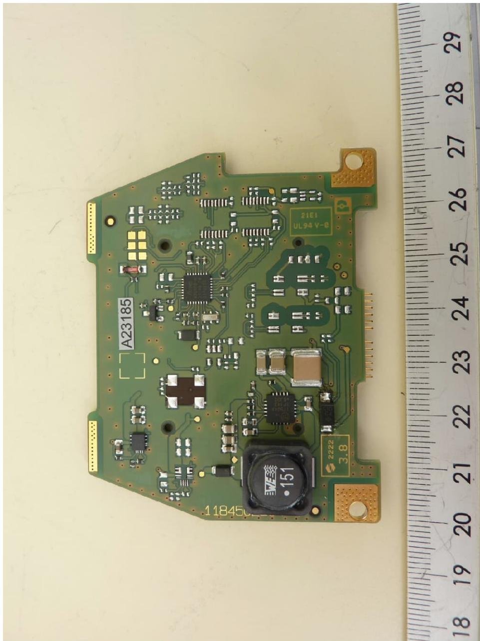
NEARFI P 2A B, data PCB, bottom view
