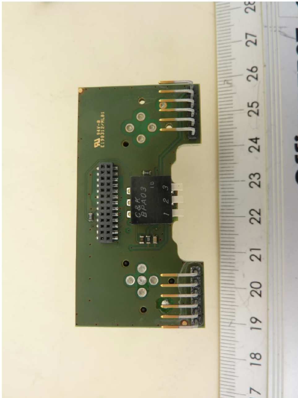
NEARFI P 2A B, interface PCB, bottom view
