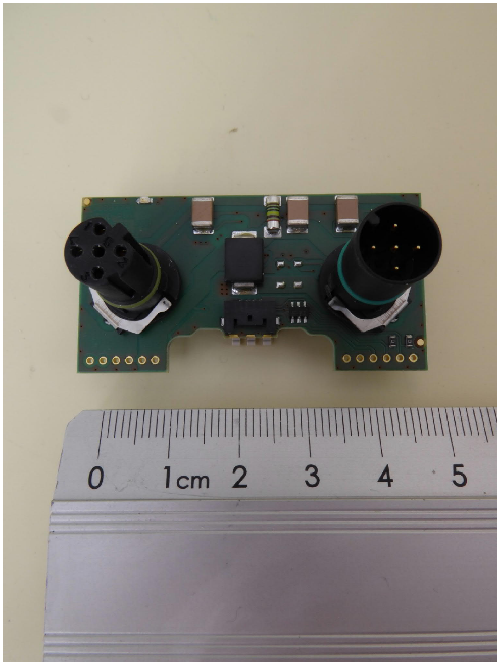
NEARFI D ETH R, interface PCB, top view
