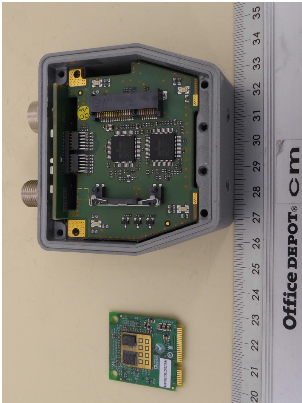
NEARFI D ETH R, internal view 3, RF-PCB removed
