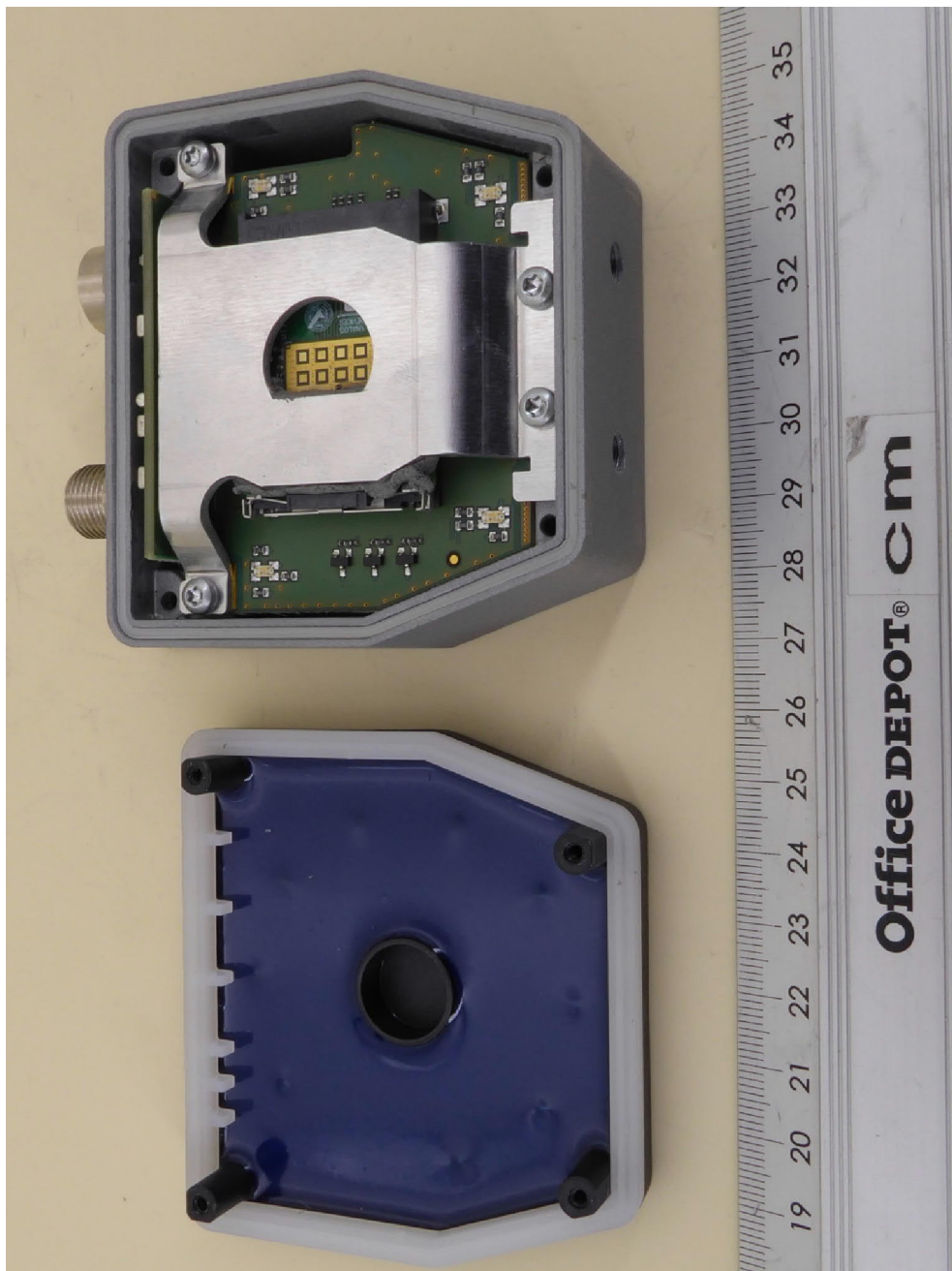
NEARFI D ETH R, internal view 1, housing opened
