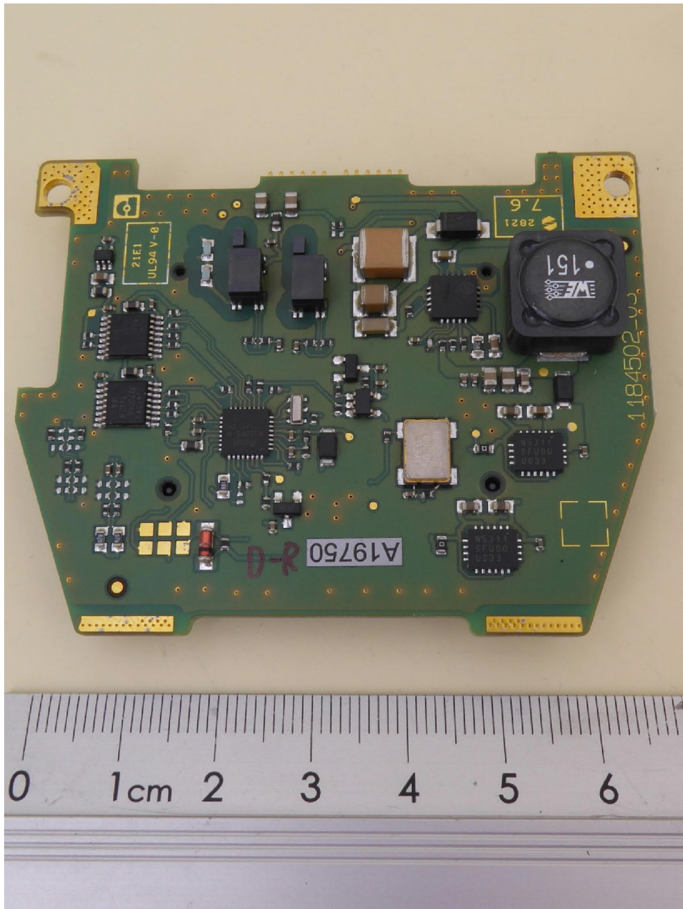
NEARFI D ETH R, data PCB, bottom view
