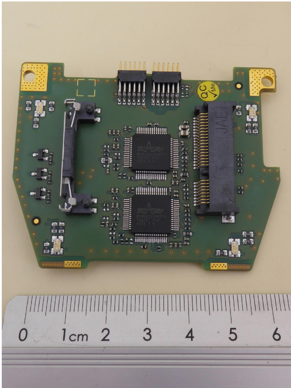
NEARFI D ETH R, data PCB, top view
