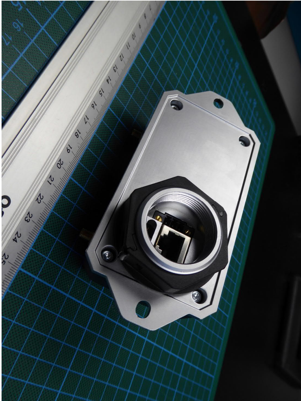
161612_DFS_M2.jpg: FL WLAN 2101, 3D view 2
