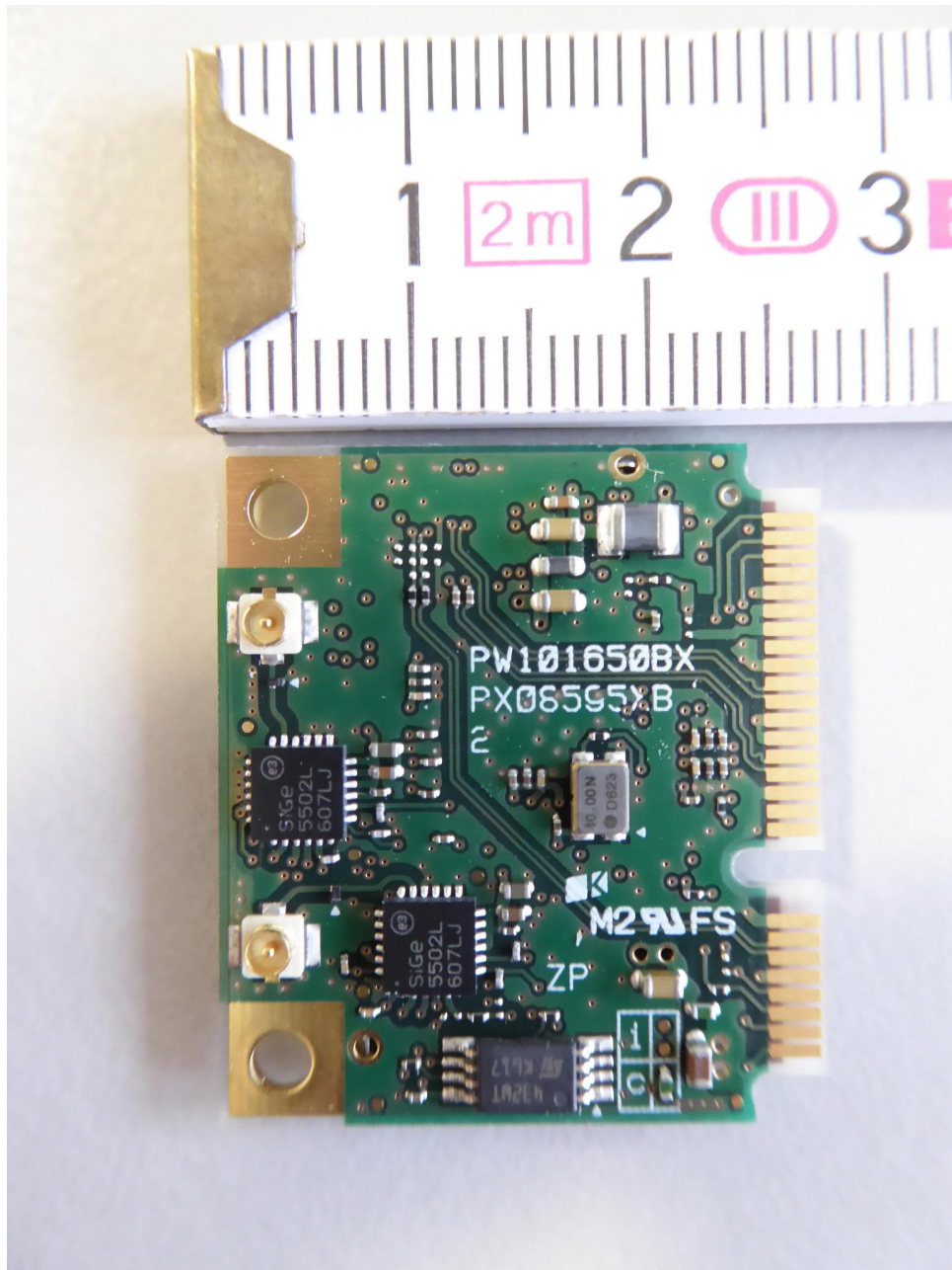
161612_DFS3.jpg: FL WLAN 2101, WLAN module, top view
