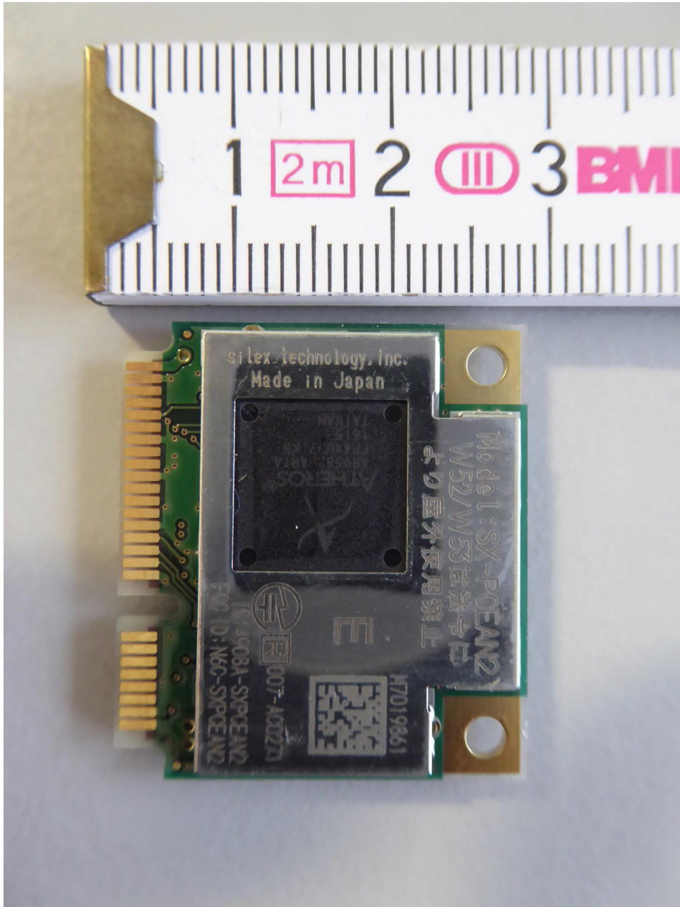
161612_DFS4.jpg: FL WLAN 2101, WLAN module, bottom view
