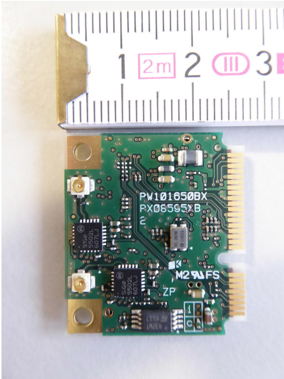
161612_DFS3.jpg: SX-PCEAN2, WLAN module, top view
