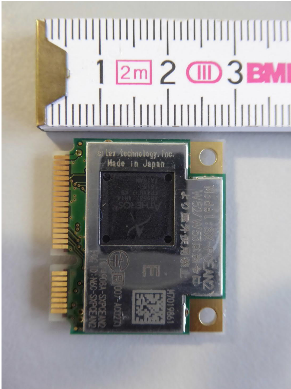
161612_DFS4.jpg: SX-PCEAN2, WLAN module, bottom view
