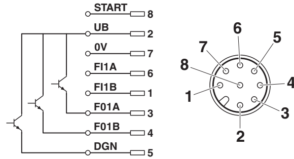
Figure 2-2 View of the connector and pin assignment
