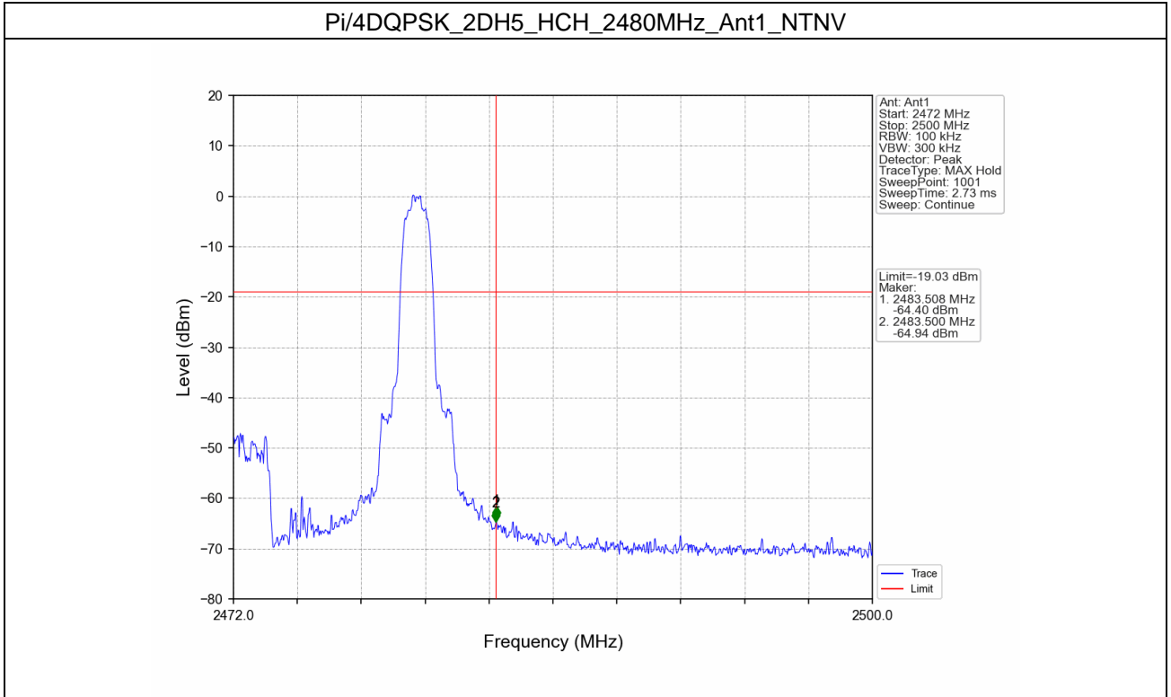
Pi/4DQPSK_2DH5_HCH_2480MHz_Ant1_NTNV
