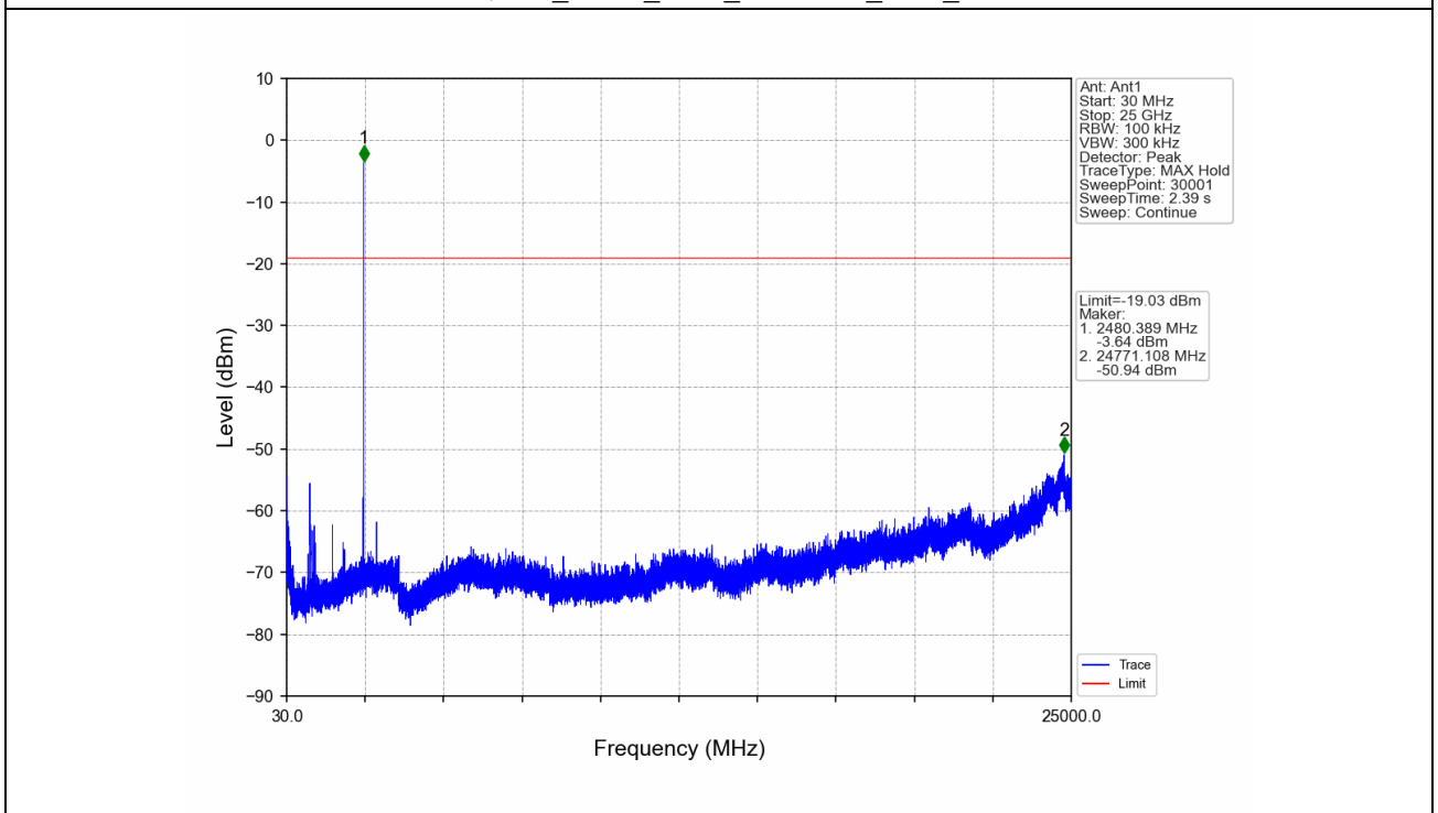
Pi/4DQPSK_2DH5_HCH_2480MHz_Ant1_NTNV
