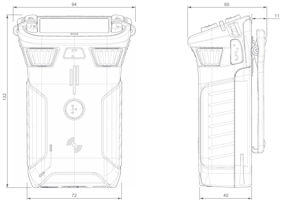
figure 204: Beltpack (front, right), dimensions in millimeter
