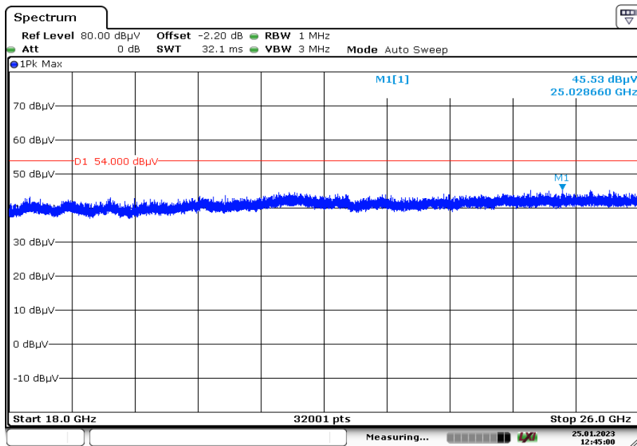
Plot 4: 18 GHz to 26 GHz, TX mode, vertical & horizontal polarization, valid for all channels
