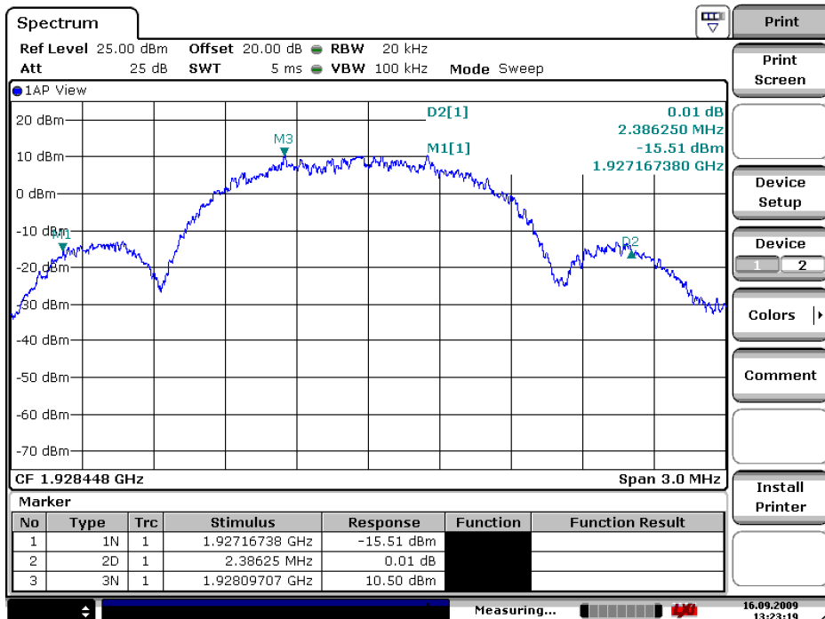
Emission Bandwidth B, Upper Channel
