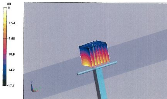
0 dB = 12.3mW/g
