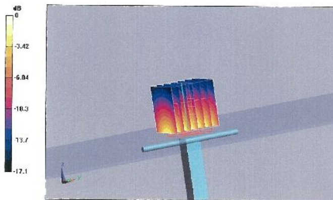
0 dB = 12.9mW/g
