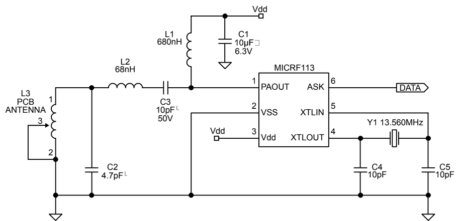
Figure 1. MICRF113 ASK Key Fob Design for 433.92 MHz
