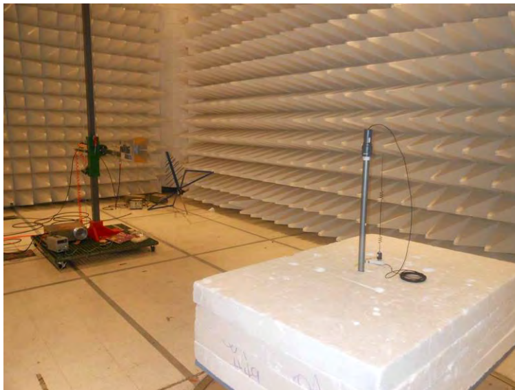
1GHz - 10GHz, 900MHz Band Antenna
