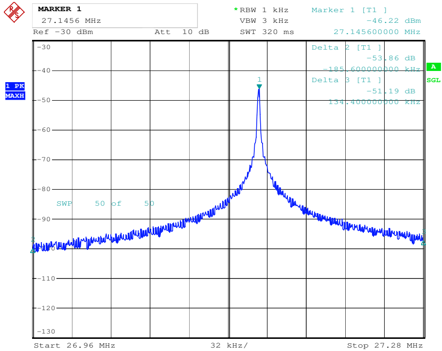
Bandwidth measurement
