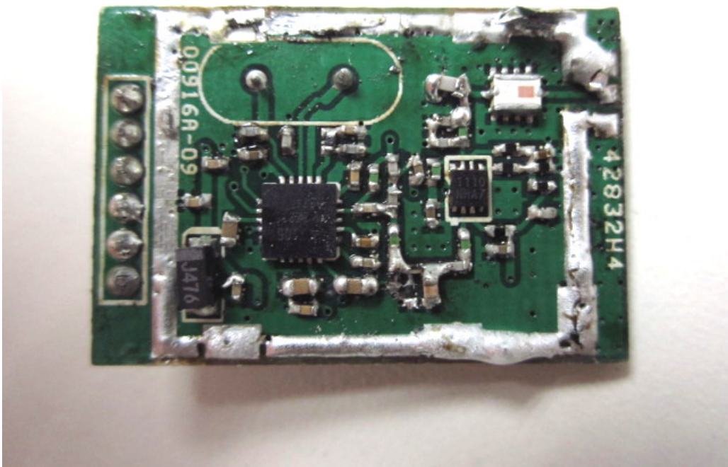
Internal View
