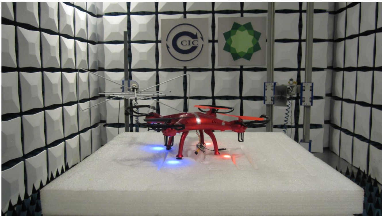
Set-up for Radiated Emission above 1GHz measurement
