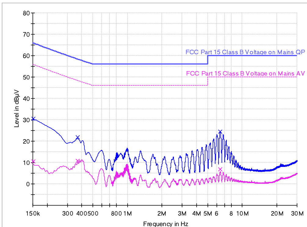
Conducted Emission (150 kHz - 30 MHz) - Cont TDS (QP+AV)
