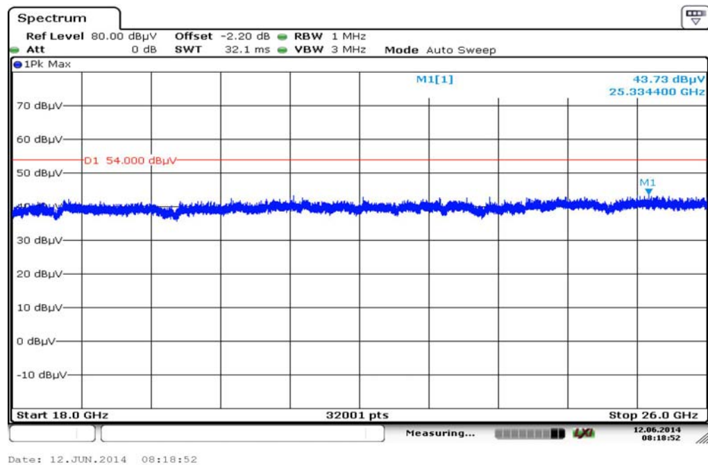
Plot 12: 18 GHz to 26 GHz, highest channel, vertical & horizontal polarization
