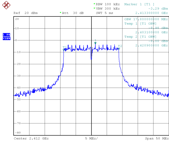
Modulation Type: 802.11n HT20 CH01
