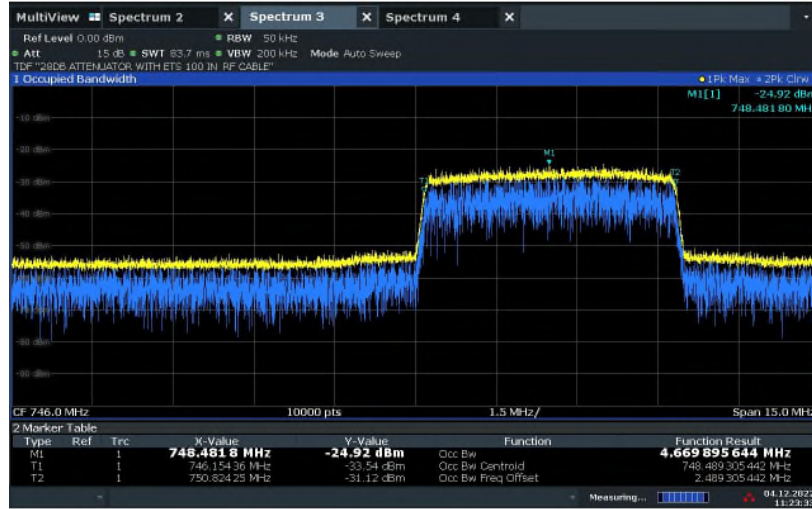
LTE B13 Downlink Low Channel OBW @ 30°C Nominal Voltage
