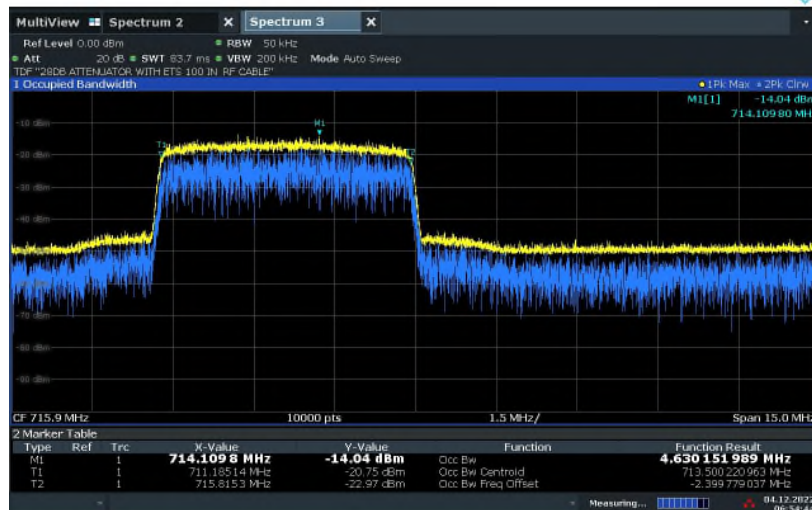
LTE B12 Uplink High Channel OBW @ 20°C Nominal Voltage
